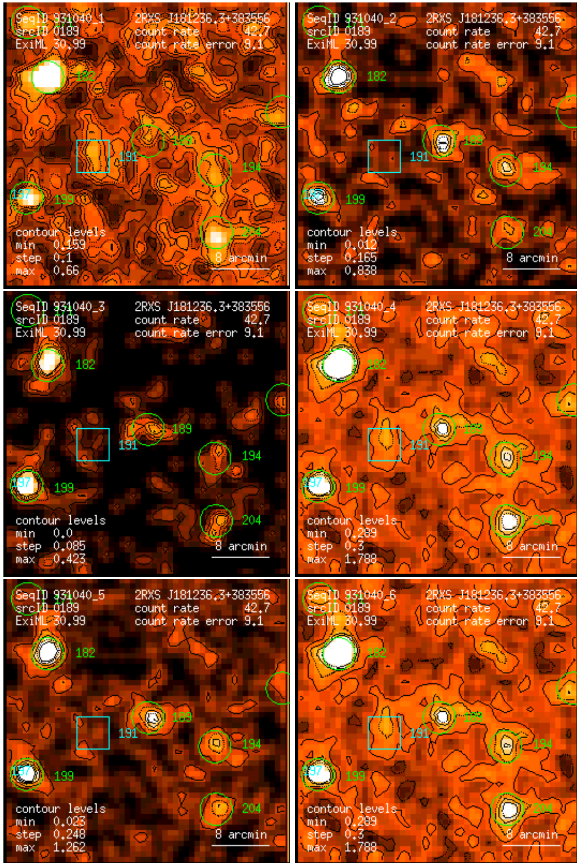
Figure 189: RASS 931040: detection 0189: band rate images, Gaussian filter: (1) PSPC channels 11 – 41, (2) 52 – 90, (3) 91 – 201, (4) 11 – 235, (5) 52 – 201, (6) 11 – 201. Broad band rates in counts/ks. Band rate contour levels in counts/ks/arcmin 2 .
