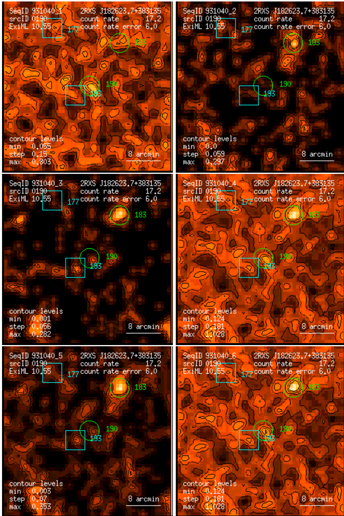
Figure 190: RASS 931040: detection 0190: band rate images, Gaussian filter: (1) PSPC channels 11 – 41, (2) 52 – 90, (3) 91 – 201, (4) 11 – 235, (5) 52 – 201, (6) 11 – 201. Broad band rates in counts/ks. Band rate contour levels in counts/ks/arcmin 2 .
