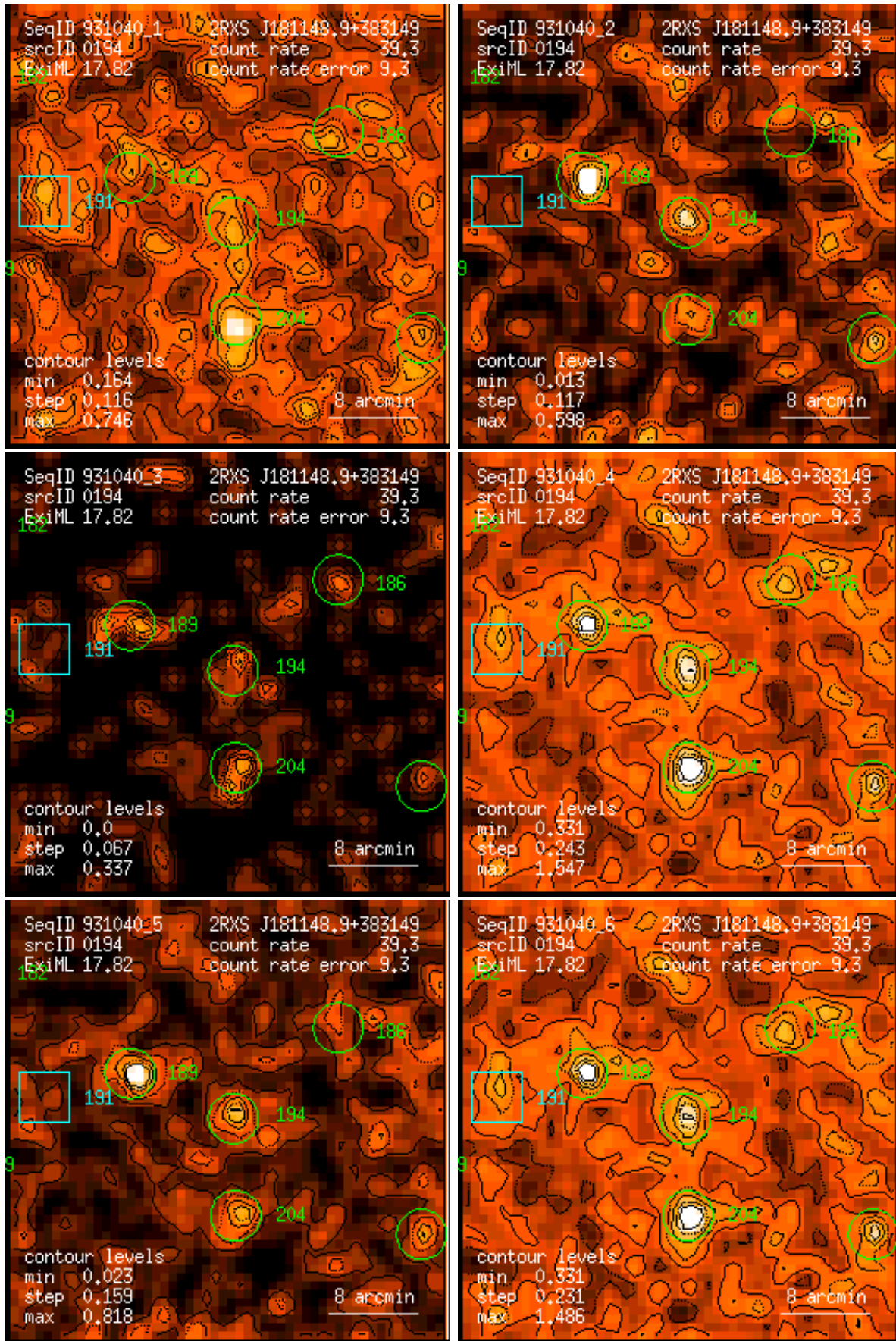
Figure 194: RASS 931040: detection 0194: band rate images, Gaussian filter: (1) PSPC channels 11 – 41, (2) 52 – 90, (3) 91 – 201, (4) 11 – 235, (5) 52 – 201, (6) 11 – 201. Broad band rates in counts/ks. Band rate contour levels in counts/ks/arcmin 2 .
