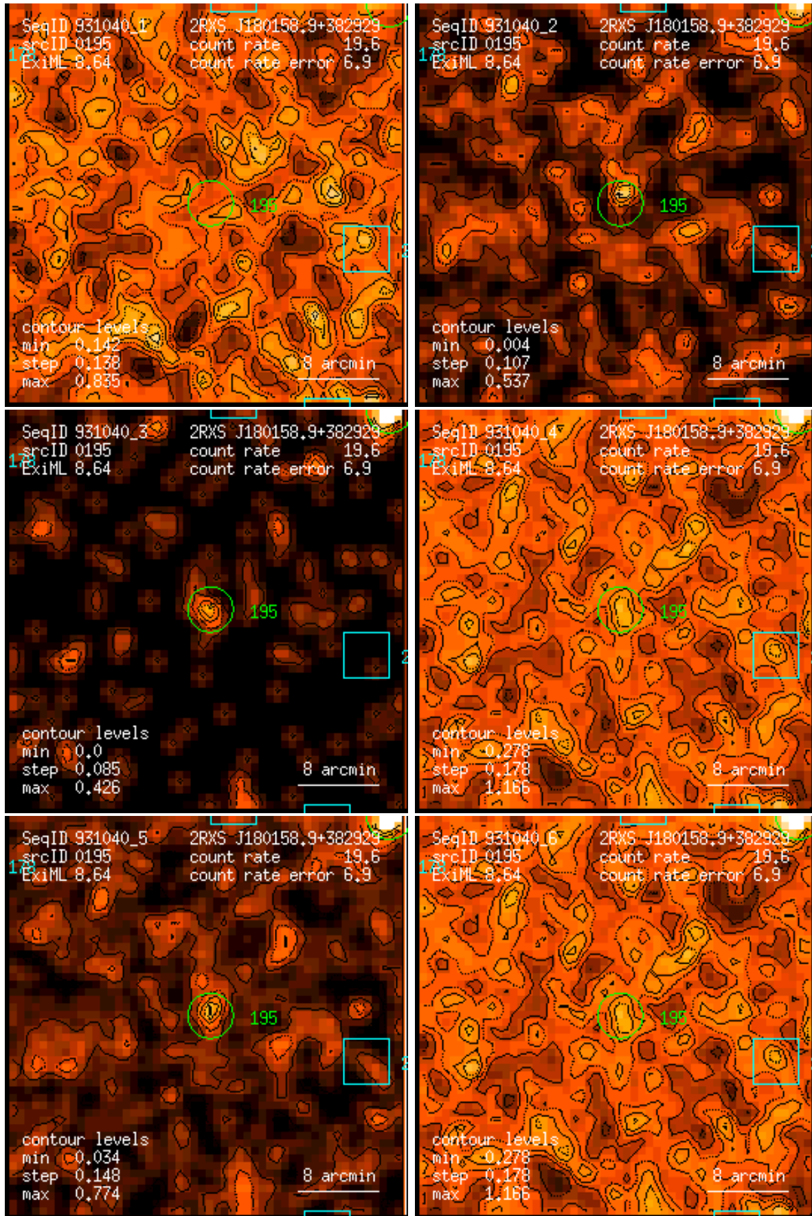
Figure 195: RASS 931040: detection 0195: band rate images, Gaussian filter: (1) PSPC channels 11 – 41, (2) 52 – 90, (3) 91 – 201, (4) 11 – 235, (5) 52 – 201, (6) 11 – 201. Broad band rates in counts/ks. Band rate contour levels in counts/ks/arcmin 2 .
