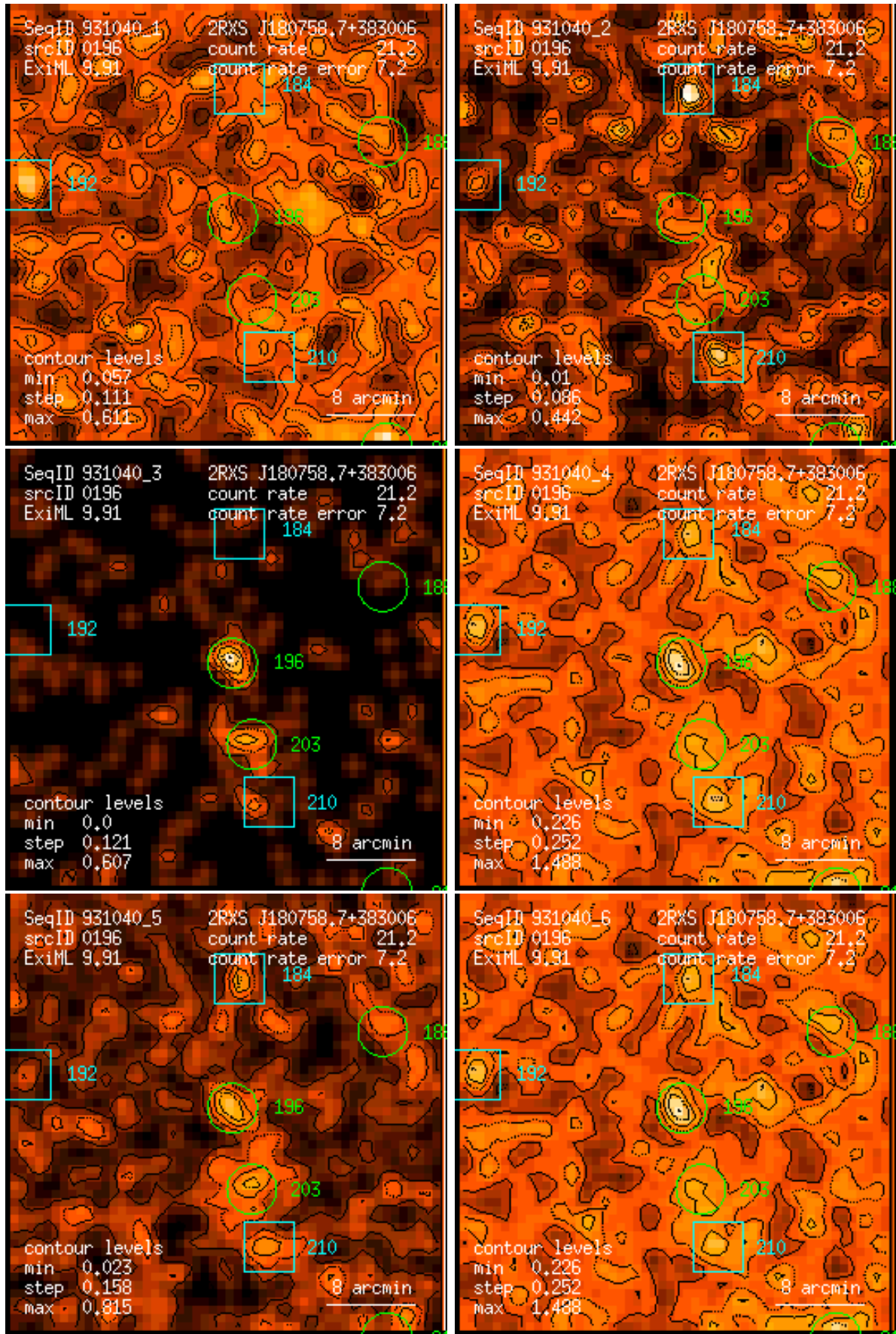
Figure 196: RASS 931040: detection 0196: band rate images, Gaussian filter: (1) PSPC channels 11 – 41, (2) 52 – 90, (3) 91 – 201, (4) 11 – 235, (5) 52 – 201, (6) 11 – 201. Broad band rates in counts/ks. Band rate contour levels in counts/ks/arcmin 2 .
