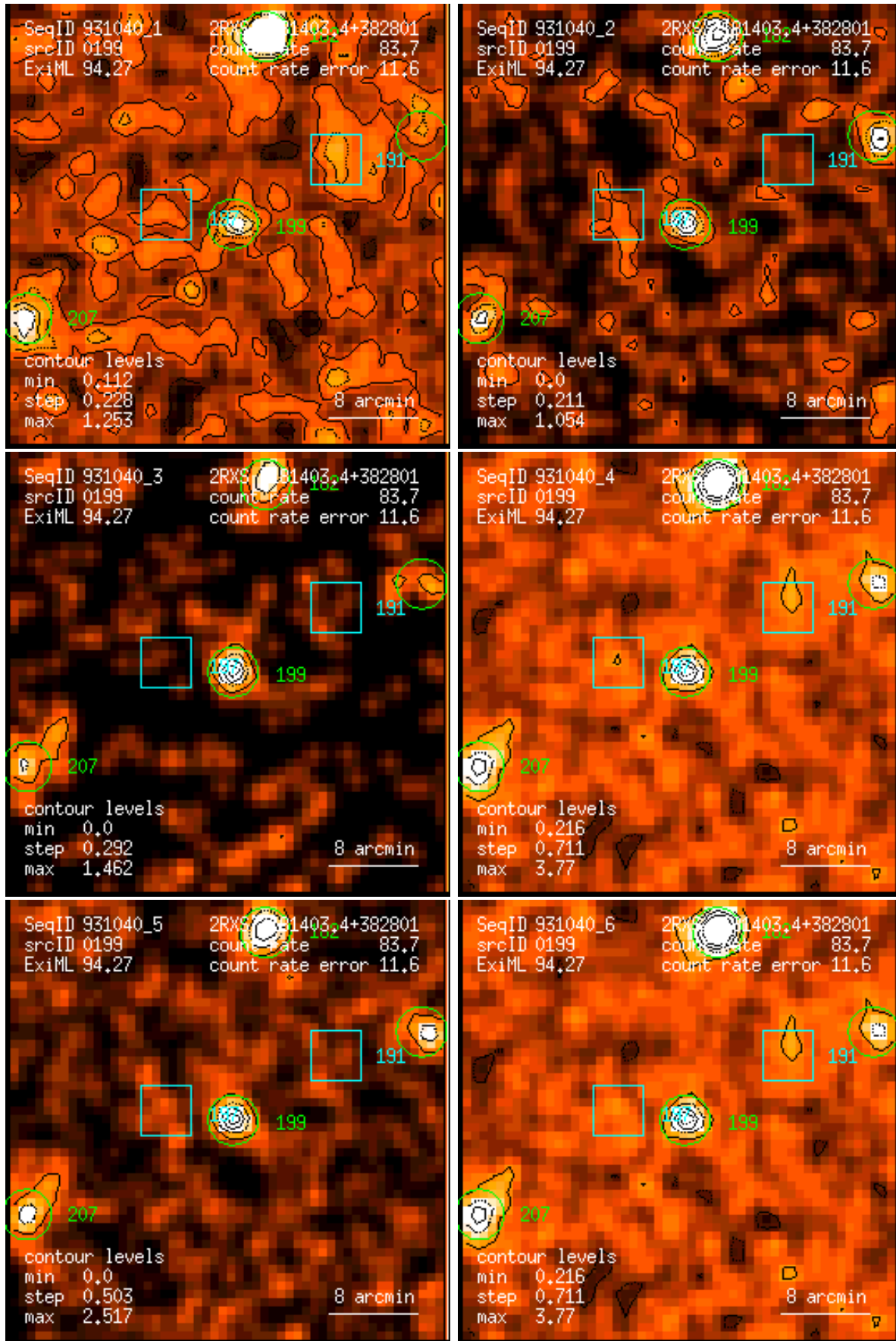
Figure 199: RASS 931040: detection 0199: band rate images, Gaussian filter: (1) PSPC channels 11 – 41, (2) 52 – 90, (3) 91 – 201, (4) 11 – 235, (5) 52 – 201, (6) 11 – 201. Broad band rates in counts/ks. Band rate contour levels in counts/ks/arcmin 2 .
