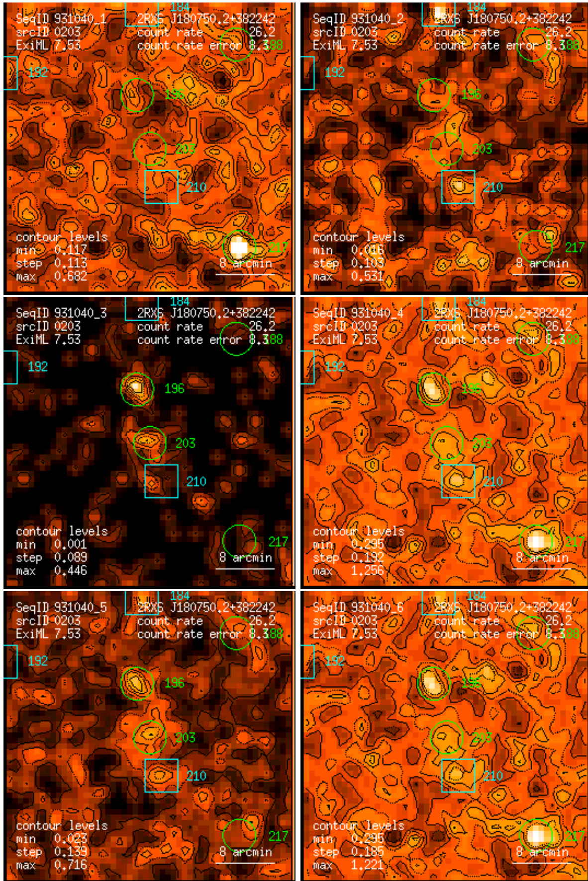
Figure 203: RASS 931040: detection 0203: band rate images, Gaussian filter: (1) PSPC channels 11 – 41, (2) 52 – 90, (3) 91 – 201, (4) 11 – 235, (5) 52 – 201, (6) 11 – 201. Broad band rates in counts/ks. Band rate contour levels in counts/ks/arcmin 2 .
