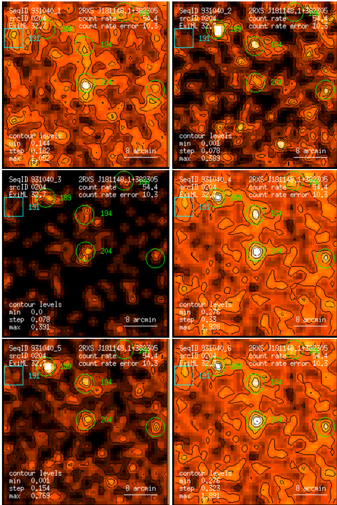
Figure 204: RASS 931040: detection 0204: band rate images, Gaussian filter: (1) PSPC channels 11 – 41, (2) 52 – 90, (3) 91 – 201, (4) 11 – 235, (5) 52 – 201, (6) 11 – 201. Broad band rates in counts/ks. Band rate contour levels in counts/ks/arcmin 2 .
