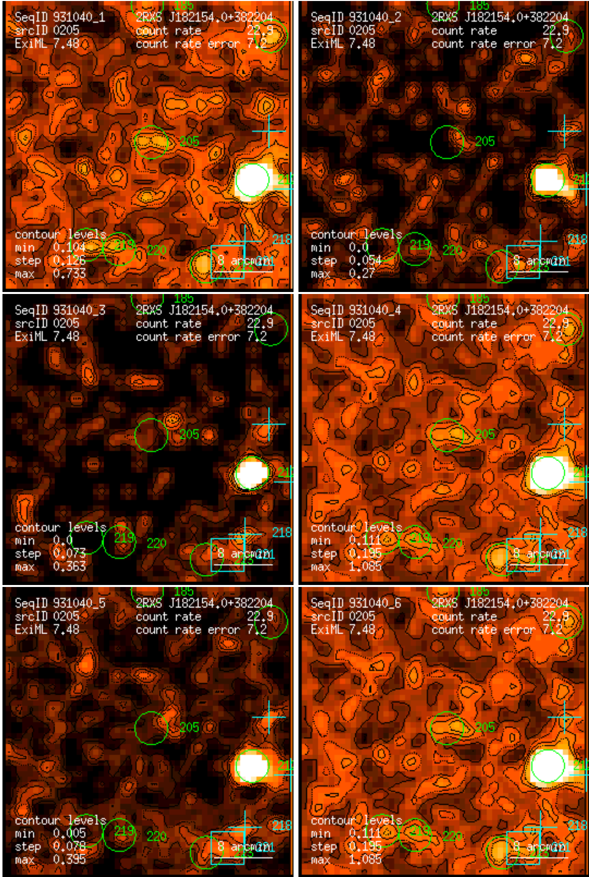
Figure 205: RASS 931040: detection 0205: band rate images, Gaussian filter: (1) PSPC channels 11 – 41, (2) 52 – 90, (3) 91 – 201, (4) 11 – 235, (5) 52 – 201, (6) 11 – 201. Broad band rates in counts/ks. Band rate contour levels in counts/ks/arcmin 2 .
