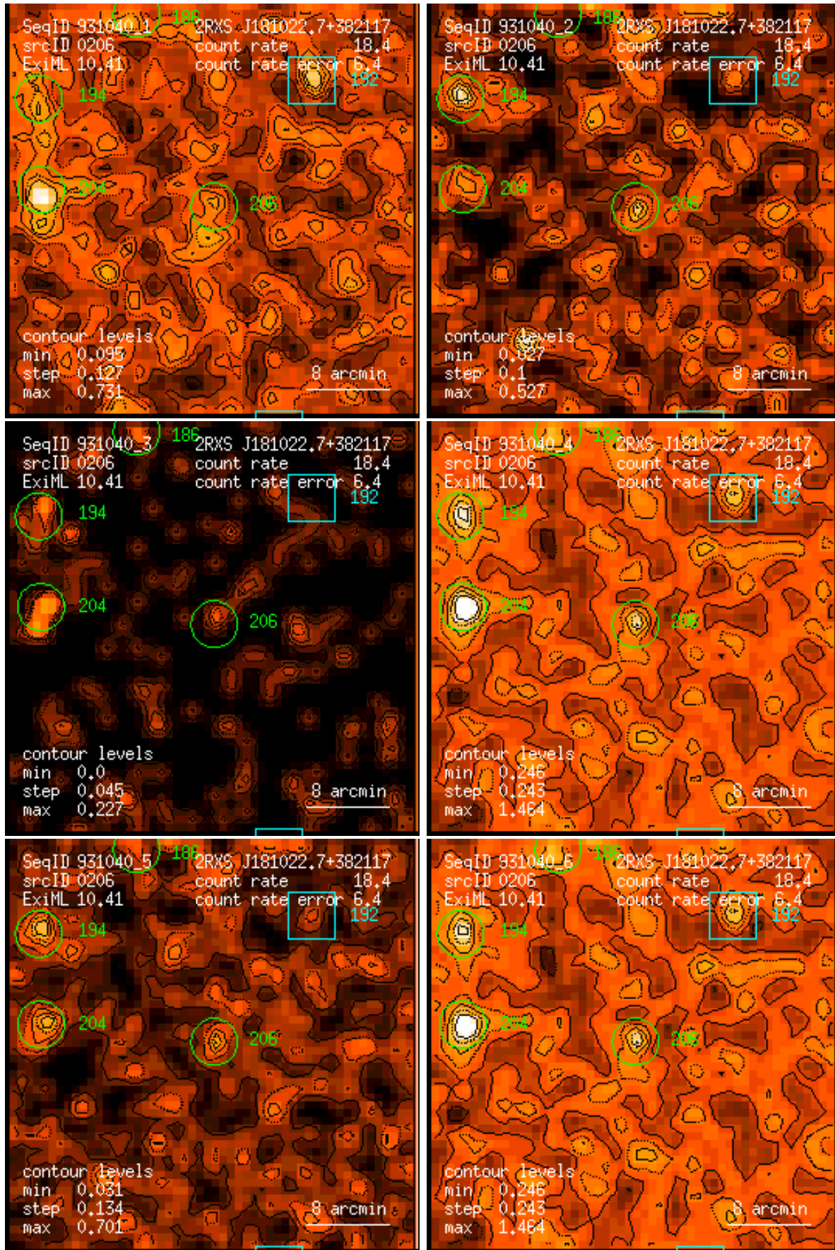
Figure 206: RASS 931040: detection 0206: band rate images, Gaussian filter: (1) PSPC channels 11 – 41, (2) 52 – 90, (3) 91 – 201, (4) 11 – 235, (5) 52 – 201, (6) 11 – 201. Broad band rates in counts/ks. Band rate contour levels in counts/ks/arcmin 2 .
