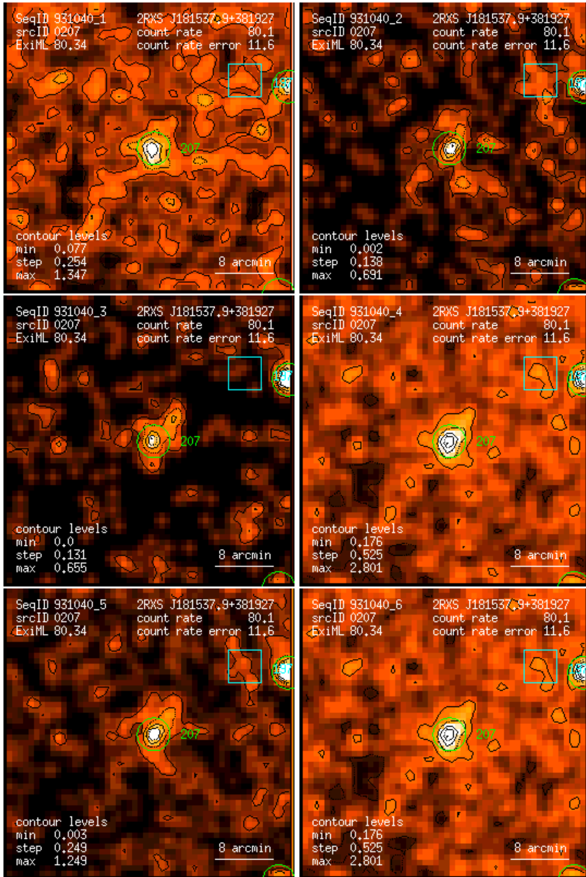
Figure 207: RASS 931040: detection 0207: band rate images, Gaussian filter: (1) PSPC channels 11 – 41, (2) 52 – 90, (3) 91 – 201, (4) 11 – 235, (5) 52 – 201, (6) 11 – 201. Broad band rates in counts/ks. Band rate contour levels in counts/ks/arcmin 2 .
