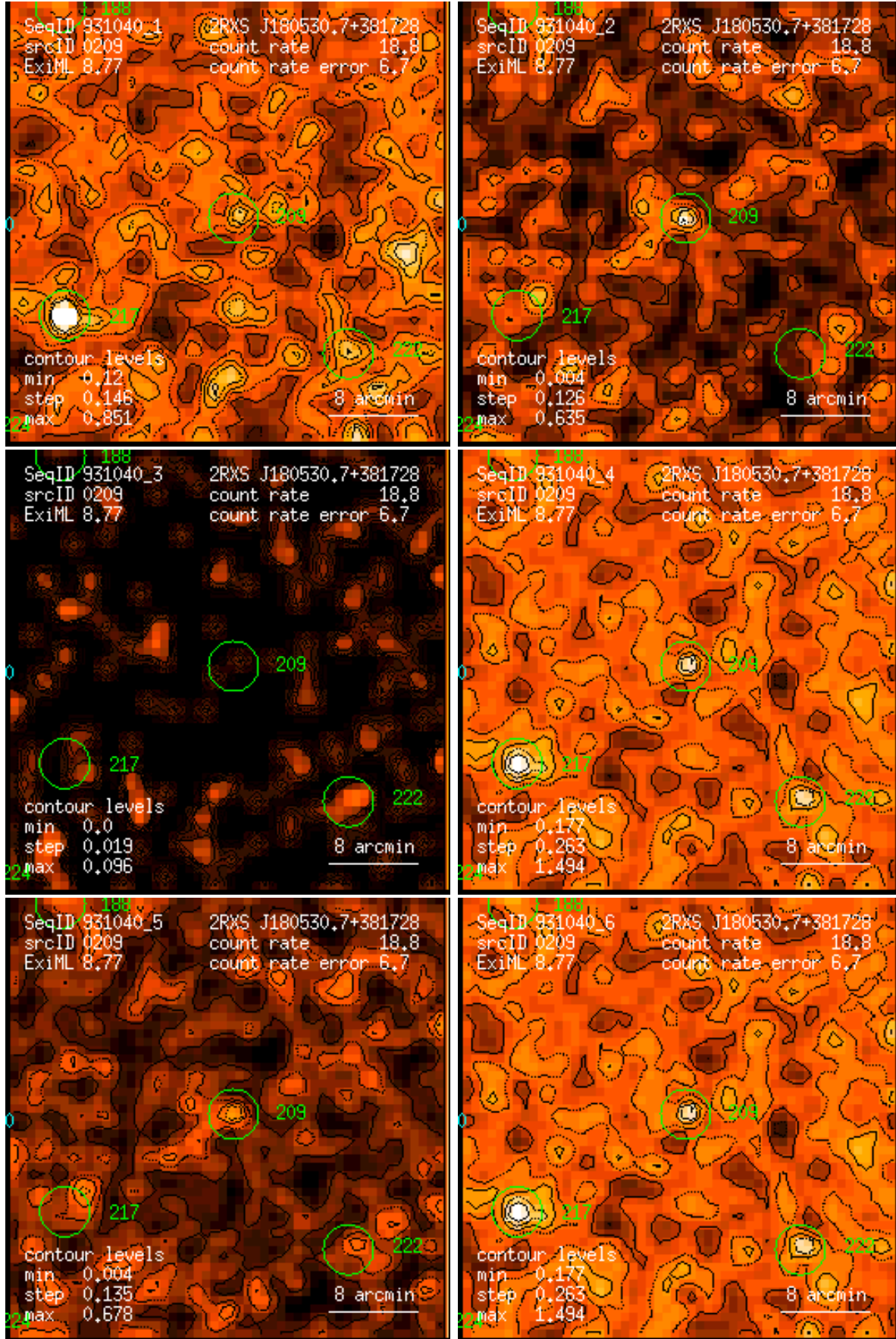
Figure 209: RASS 931040: detection 0209: band rate images, Gaussian filter: (1) PSPC channels 11 – 41, (2) 52 – 90, (3) 91 – 201, (4) 11 – 235, (5) 52 – 201, (6) 11 – 201. Broad band rates in counts/ks. Band rate contour levels in counts/ks/arcmin 2 .
