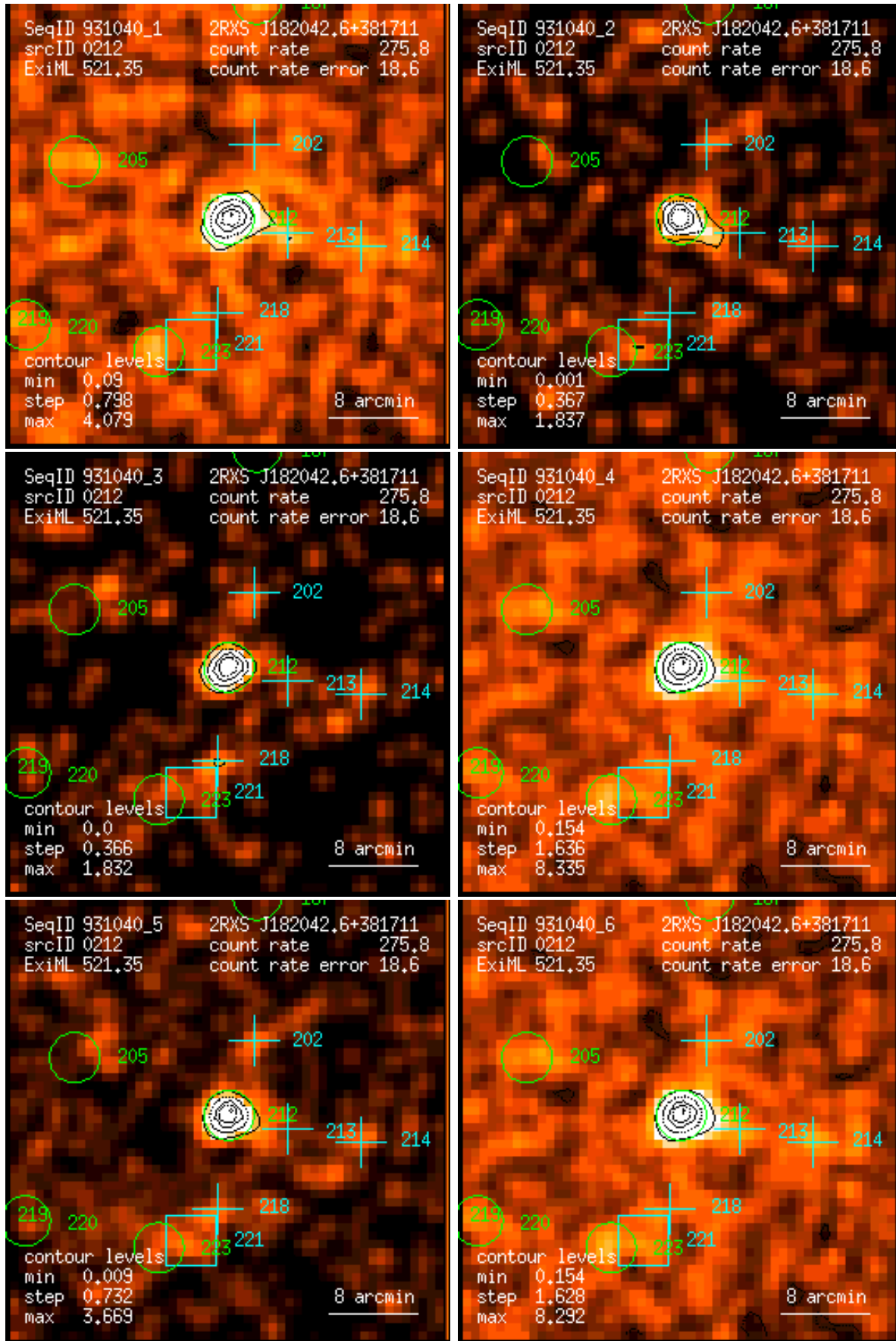
Figure 212: RASS 931040: detection 0212: band rate images, Gaussian filter: (1) PSPC channels 11 – 41, (2) 52 – 90, (3) 91 – 201, (4) 11 – 235, (5) 52 – 201, (6) 11 – 201. Broad band rates in counts/ks. Band rate contour levels in counts/ks/arcmin 2 .
