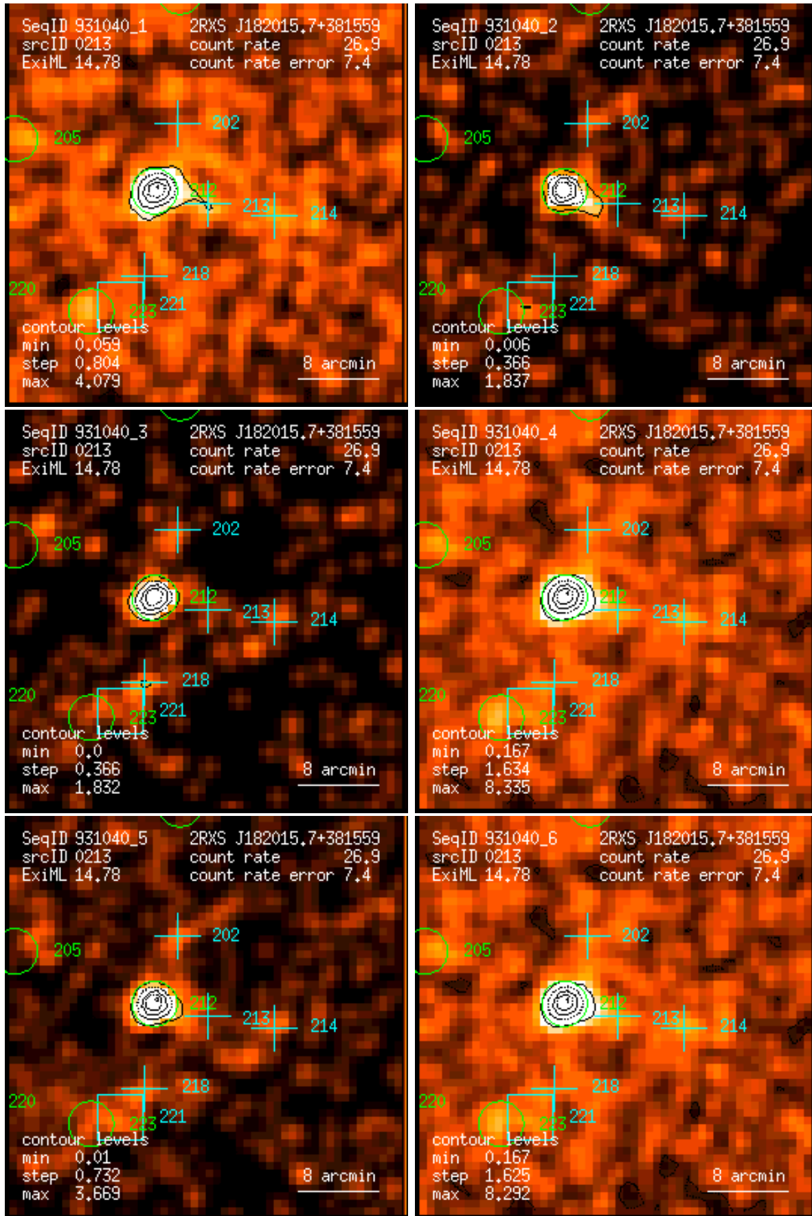
Figure 213: RASS 931040: detection 0213: band rate images, Gaussian filter: (1) PSPC channels 11 – 41, (2) 52 – 90, (3) 91 – 201, (4) 11 – 235, (5) 52 – 201, (6) 11 – 201. Broad band rates in counts/ks. Band rate contour levels in counts/ks/arcmin 2 .
