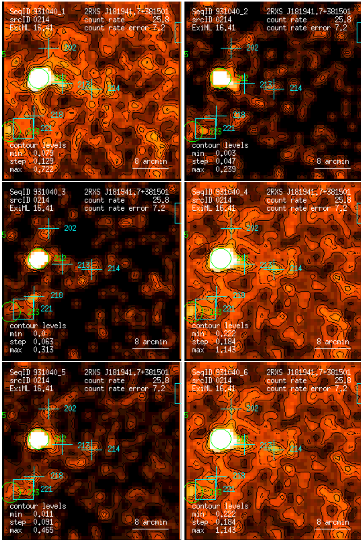
Figure 214: RASS 931040: detection 0214: band rate images, Gaussian filter: (1) PSPC channels 11 – 41, (2) 52 – 90, (3) 91 – 201, (4) 11 – 235, (5) 52 – 201, (6) 11 – 201. Broad band rates in counts/ks. Band rate contour levels in counts/ks/arcmin 2 .
