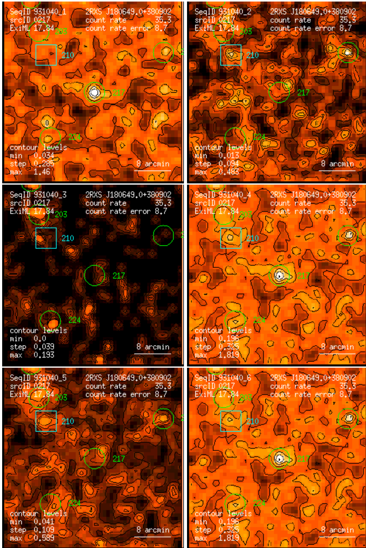
Figure 217: RASS 931040: detection 0217: band rate images, Gaussian filter: (1) PSPC channels 11 – 41, (2) 52 – 90, (3) 91 – 201, (4) 11 – 235, (5) 52 – 201, (6) 11 – 201. Broad band rates in counts/ks. Band rate contour levels in counts/ks/arcmin 2 .
