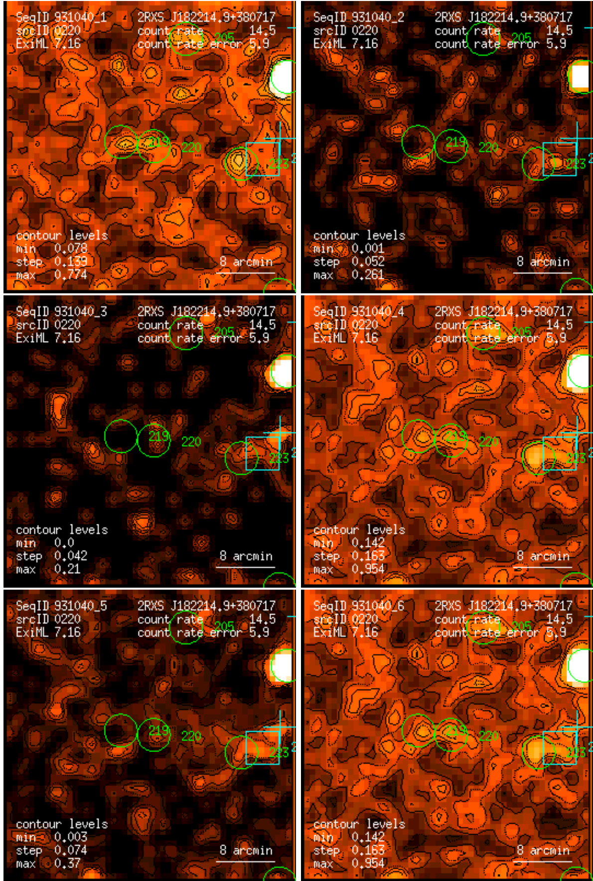
Figure 220: RASS 931040: detection 0220: band rate images, Gaussian filter: (1) PSPC channels 11 – 41, (2) 52 – 90, (3) 91 – 201, (4) 11 – 235, (5) 52 – 201, (6) 11 – 201. Broad band rates in counts/ks. Band rate contour levels in counts/ks/arcmin 2 .
