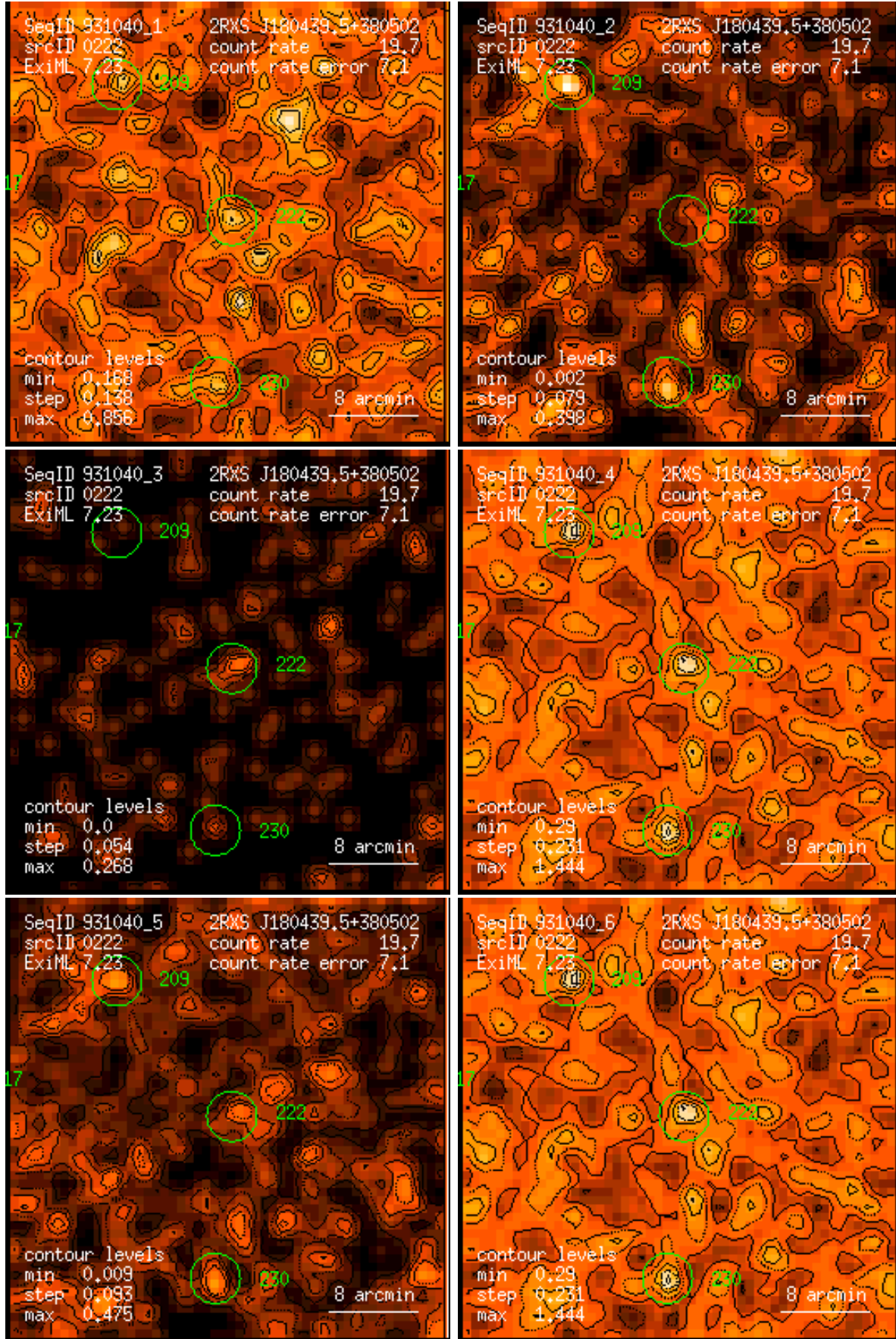
Figure 222: RASS 931040: detection 0222: band rate images, Gaussian filter: (1) PSPC channels 11 – 41, (2) 52 – 90, (3) 91 – 201, (4) 11 – 235, (5) 52 – 201, (6) 11 – 201. Broad band rates in counts/ks. Band rate contour levels in counts/ks/arcmin 2 .
