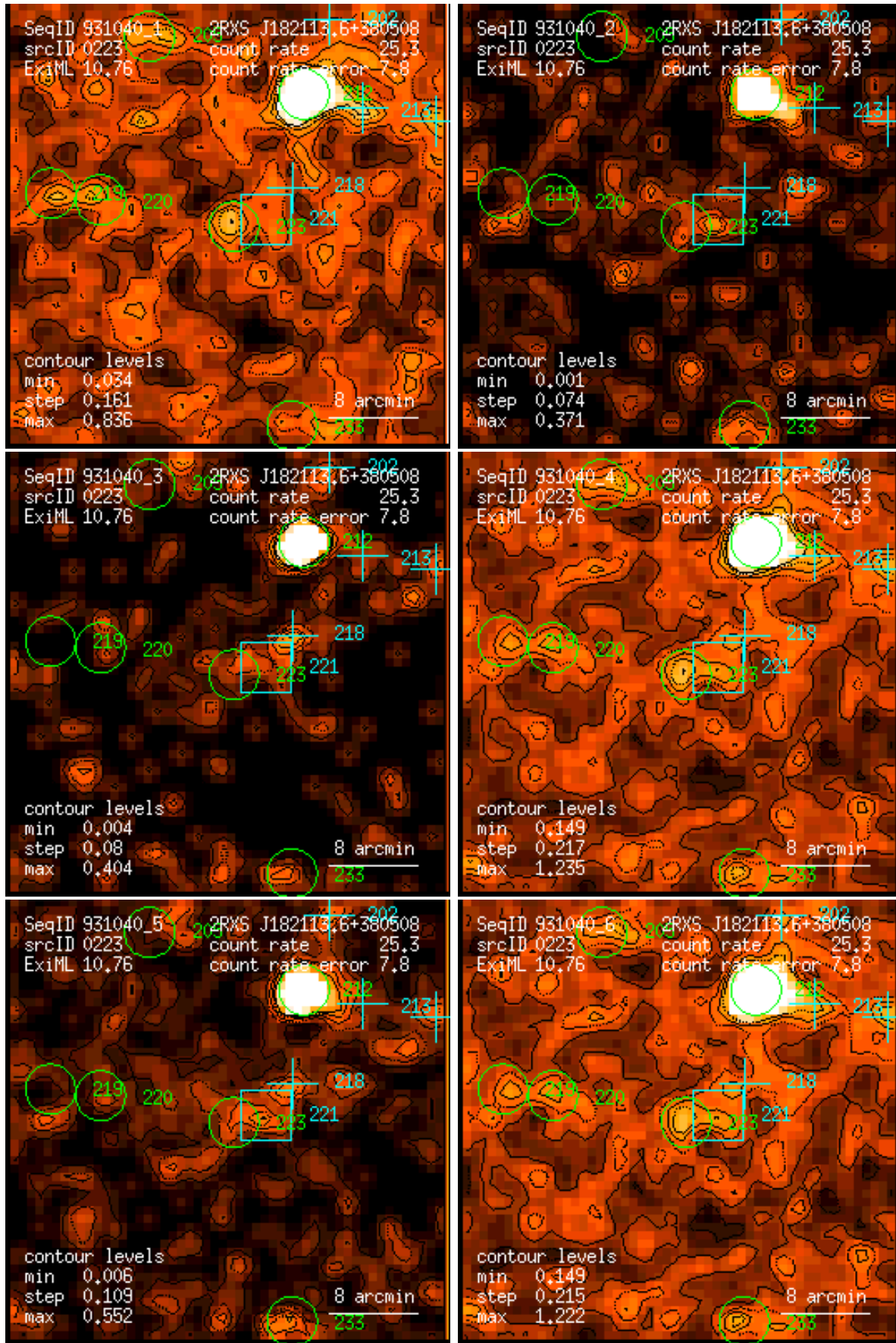
Figure 223: RASS 931040: detection 0223: band rate images, Gaussian filter: (1) PSPC channels 11 – 41, (2) 52 – 90, (3) 91 – 201, (4) 11 – 235, (5) 52 – 201, (6) 11 – 201. Broad band rates in counts/ks. Band rate contour levels in counts/ks/arcmin 2 .
