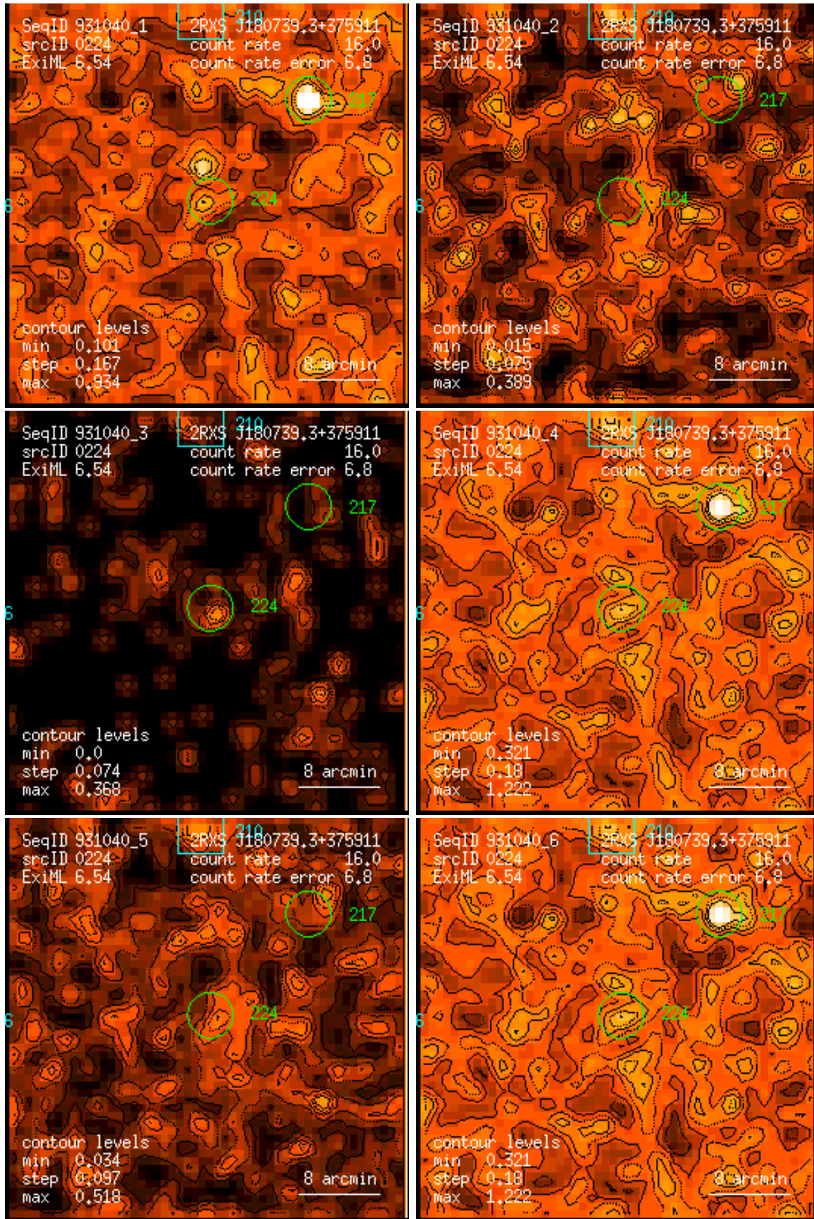
Figure 224: RASS 931040: detection 0224: band rate images, Gaussian filter: (1) PSPC channels 11 – 41, (2) 52 – 90, (3) 91 – 201, (4) 11 – 235, (5) 52 – 201, (6) 11 – 201. Broad band rates in counts/ks. Band rate contour levels in counts/ks/arcmin 2 .
