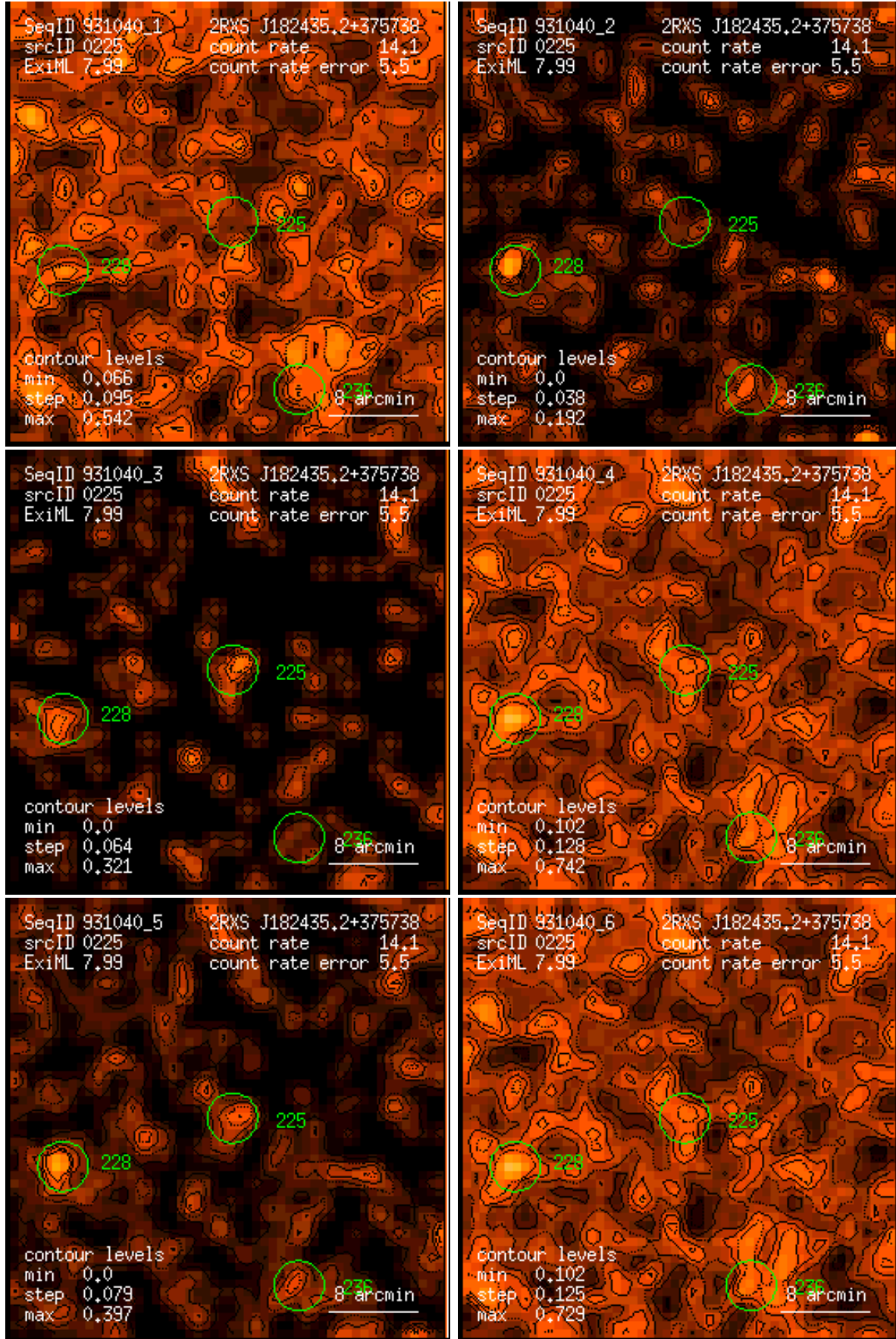
Figure 225: RASS 931040: detection 0225: band rate images, Gaussian filter: (1) PSPC channels 11 – 41, (2) 52 – 90, (3) 91 – 201, (4) 11 – 235, (5) 52 – 201, (6) 11 – 201. Broad band rates in counts/ks. Band rate contour levels in counts/ks/arcmin 2 .
