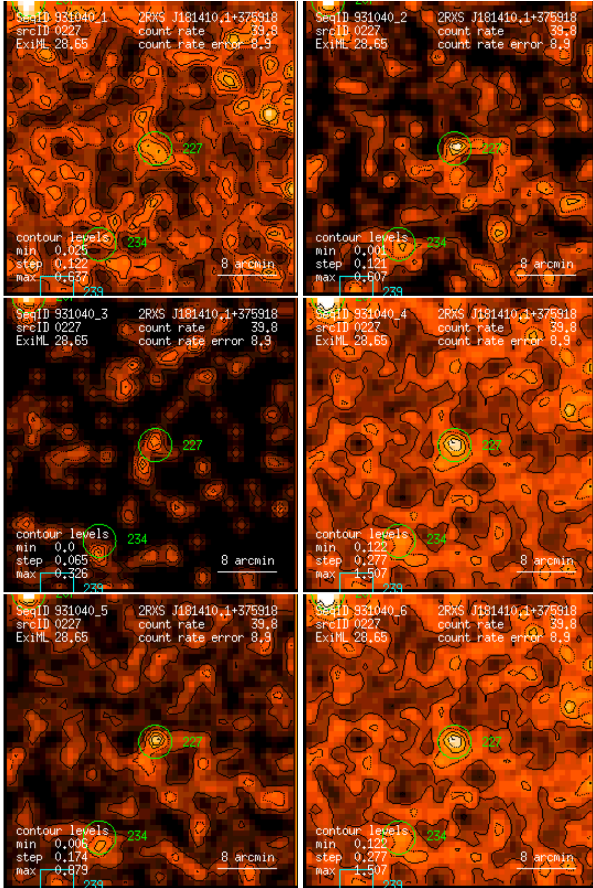
Figure 227: RASS 931040: detection 0227: band rate images, Gaussian filter: (1) PSPC channels 11 – 41, (2) 52 – 90, (3) 91 – 201, (4) 11 – 235, (5) 52 – 201, (6) 11 – 201. Broad band rates in counts/ks. Band rate contour levels in counts/ks/arcmin 2 .
