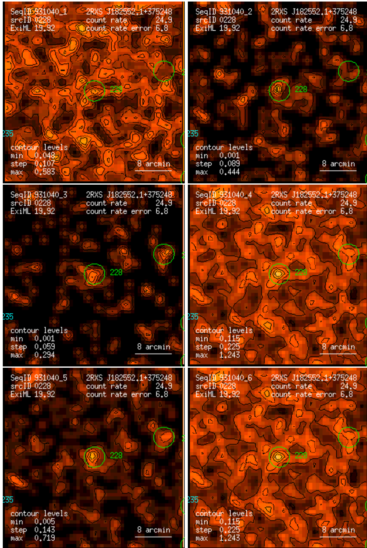
Figure 228: RASS 931040: detection 0228: band rate images, Gaussian filter: (1) PSPC channels 11 – 41, (2) 52 – 90, (3) 91 – 201, (4) 11 – 235, (5) 52 – 201, (6) 11 – 201. Broad band rates in counts/ks. Band rate contour levels in counts/ks/arcmin 2 .
