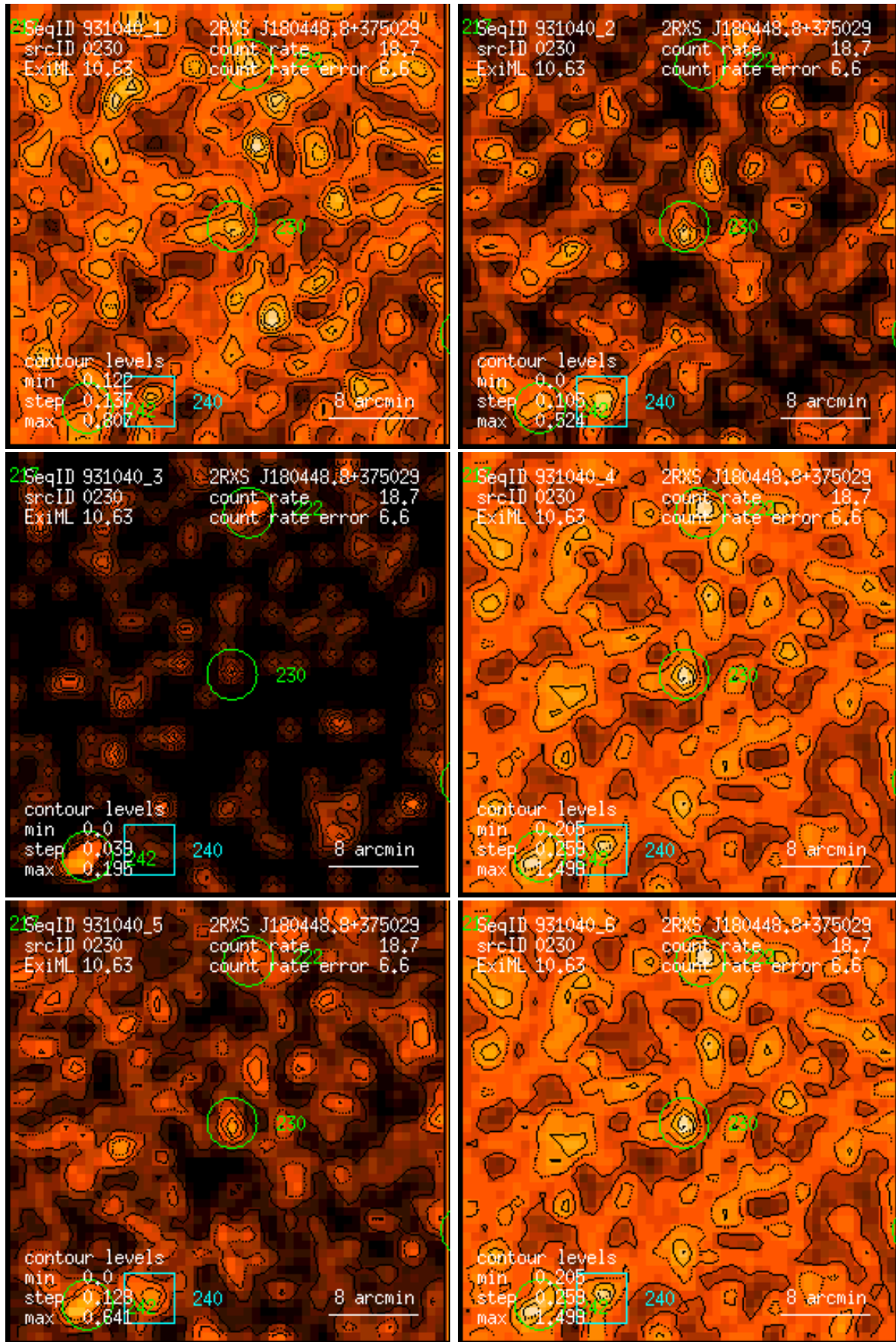
Figure 230: RASS 931040: detection 0230: band rate images, Gaussian filter: (1) PSPC channels 11 – 41, (2) 52 – 90, (3) 91 – 201, (4) 11 – 235, (5) 52 – 201, (6) 11 – 201. Broad band rates in counts/ks. Band rate contour levels in counts/ks/arcmin 2 .
