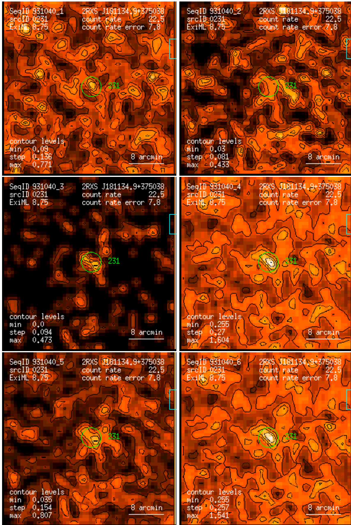
Figure 231: RASS 931040: detection 0231: band rate images, Gaussian filter: (1) PSPC channels 11 – 41, (2) 52 – 90, (3) 91 – 201, (4) 11 – 235, (5) 52 – 201, (6) 11 – 201. Broad band rates in counts/ks. Band rate contour levels in counts/ks/arcmin 2 .
