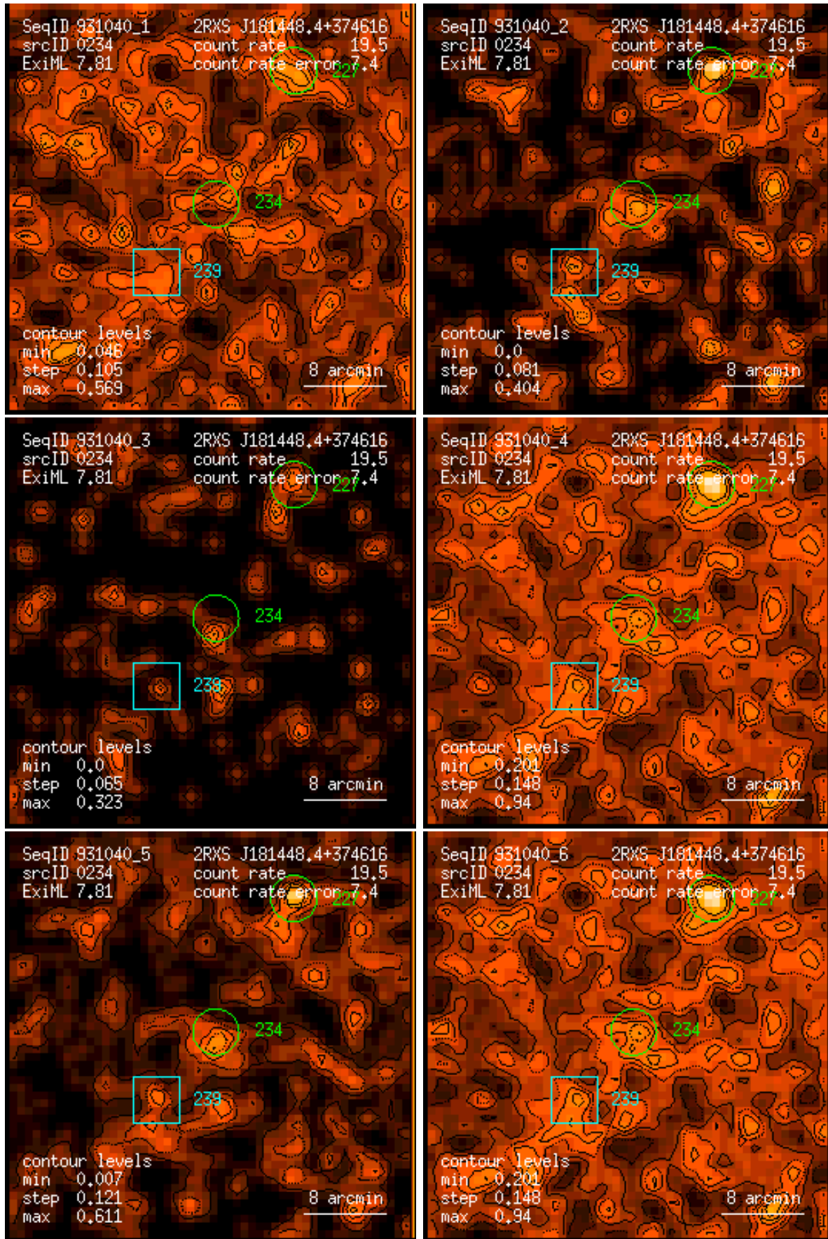
Figure 234: RASS 931040: detection 0234: band rate images, Gaussian filter: (1) PSPC channels 11 – 41, (2) 52 – 90, (3) 91 – 201, (4) 11 – 235, (5) 52 – 201, (6) 11 – 201. Broad band rates in counts/ks. Band rate contour levels in counts/ks/arcmin 2 .
