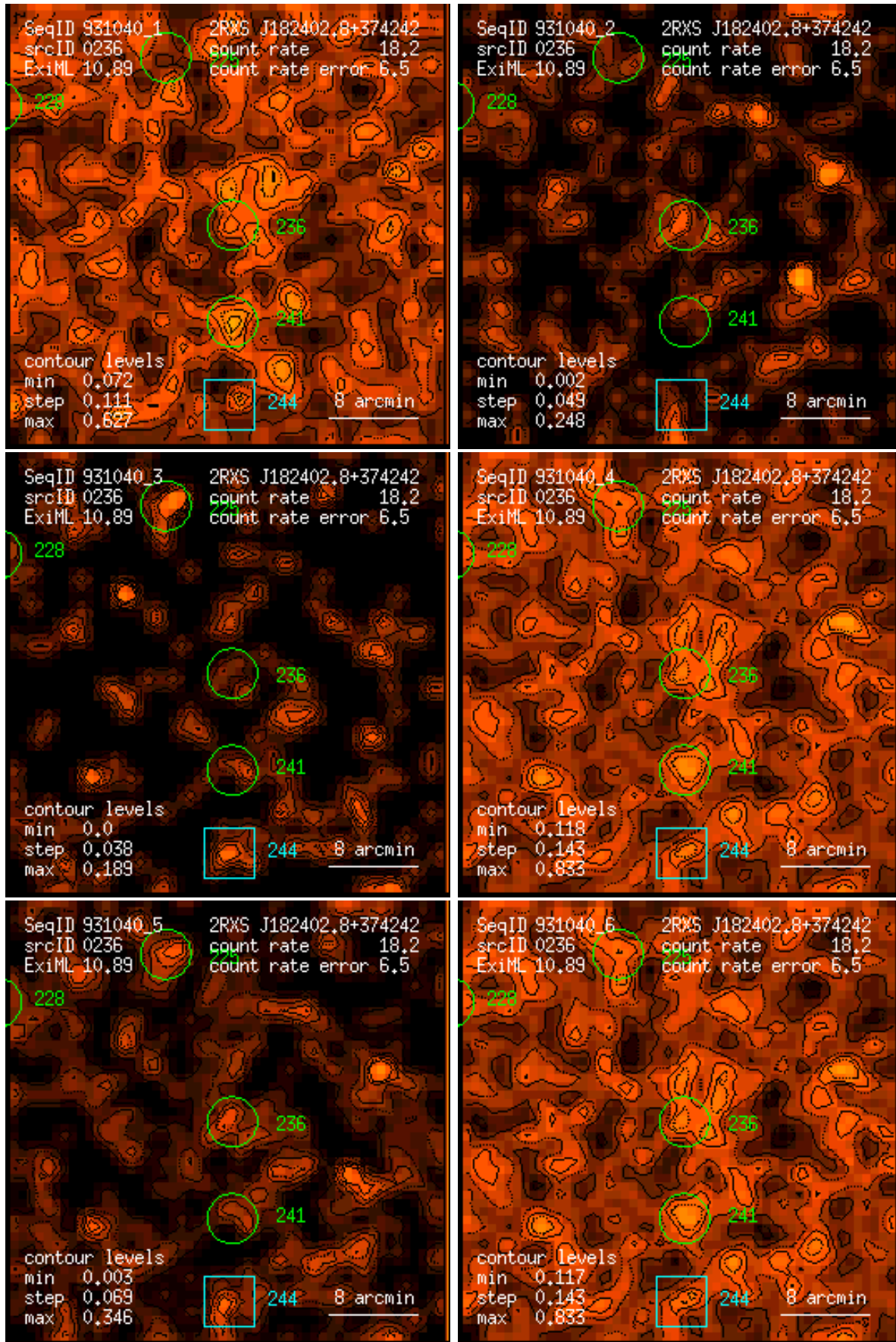
Figure 236: RASS 931040: detection 0236: band rate images, Gaussian filter: (1) PSPPC channels 11 – 41, (2) 52 – 90, (3) 91 – 201, (4) 11 – 235, (5) 52 – 201, (6) 11 – 201. Broad band rates in counts/ks. Band rate contour levels in counts/ks/arcmin 2 .
