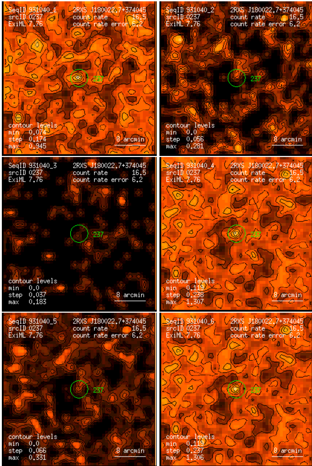
Figure 237: RASS 931040: detection 0237: band rate images, Gaussian filter: (1) PSPC channels 11 – 41, (2) 52 – 90, (3) 91 – 201, (4) 11 – 235, (5) 52 – 201, (6) 11 – 201. Broad band rates in counts/ks. Band rate contour levels in counts/ks/arcmin 2 .
