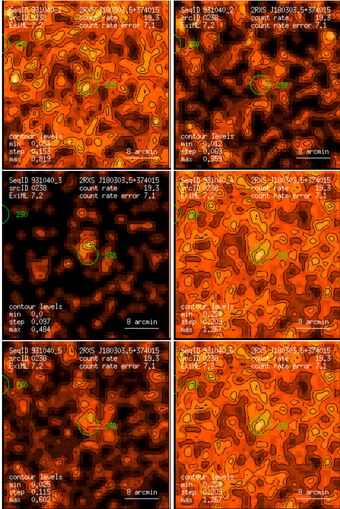
Figure 238: RASS 931040: detection 0238: band rate images, Gaussian filter: (1) PSPC channels 11 – 41, (2) 52 – 90, (3) 91 – 201, (4) 11 – 235, (5) 52 – 201, (6) 11 – 201. Broad band rates in counts/ks. Band rate contour levels in counts/ks/arcmin 2 .
