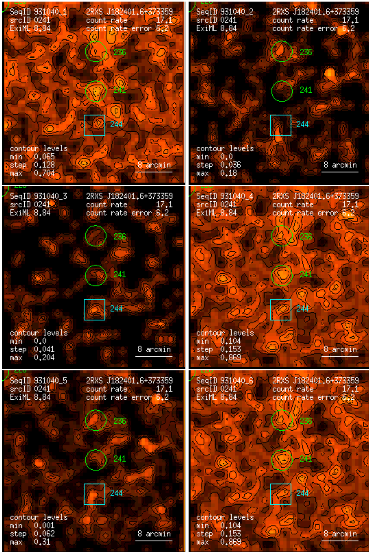
Figure 241: RASS 931040: detection 0241: band rate images, Gaussian filter: (1) PSPC channels 11 – 41, (2) 52 – 90, (3) 91 – 201, (4) 11 – 235, (5) 52 – 201, (6) 11 – 201. Broad band rates in counts/ks. Band rate contour levels in counts/ks/arcmin 2 .
