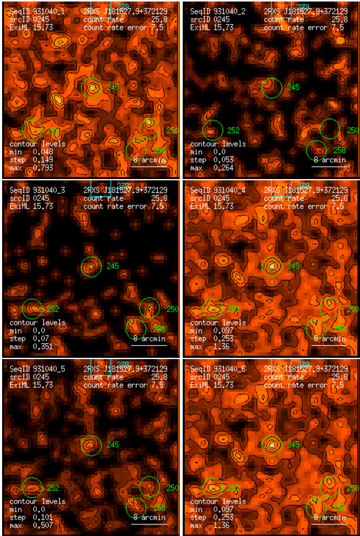
Figure 245: RASS 931040: detection 0245: band rate images, Gaussian filter: (1) PSPC channels 11 – 41, (2) 52 – 90, (3) 91 – 201, (4) 11 – 235, (5) 52 – 201, (6) 11 – 201. Broad band rates in counts/ks. Band rate contour levels in counts/ks/arcmin 2 .
