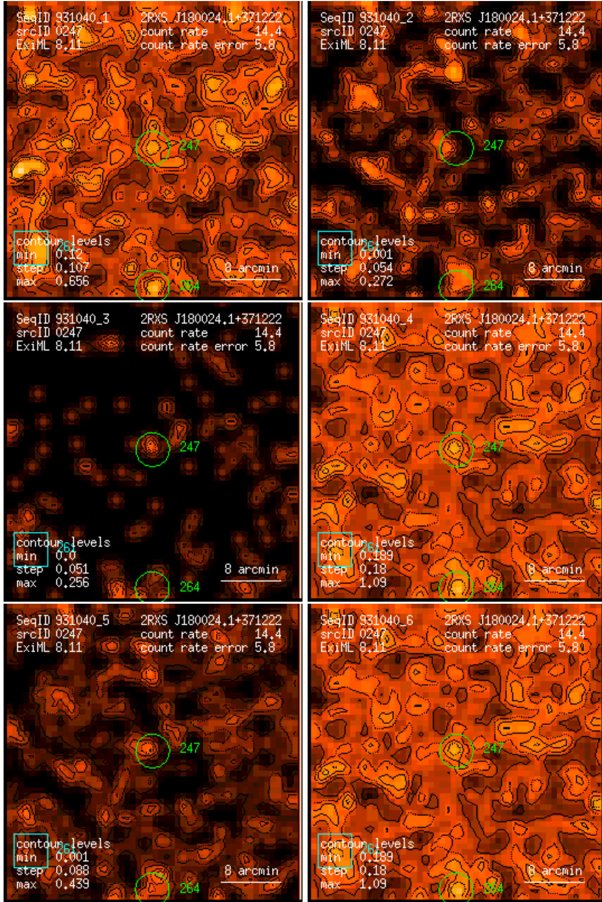
Figure 247: RASS 931040: detection 0247: band rate images, Gaussian filter: (1) PSPC channels 11 – 41, (2) 52 – 90, (3) 91 – 201, (4) 11 – 235, (5) 52 – 201, (6) 11 – 201. Broad band rates in counts/ks. Band rate contour levels in counts/ks/arcmin 2 .
