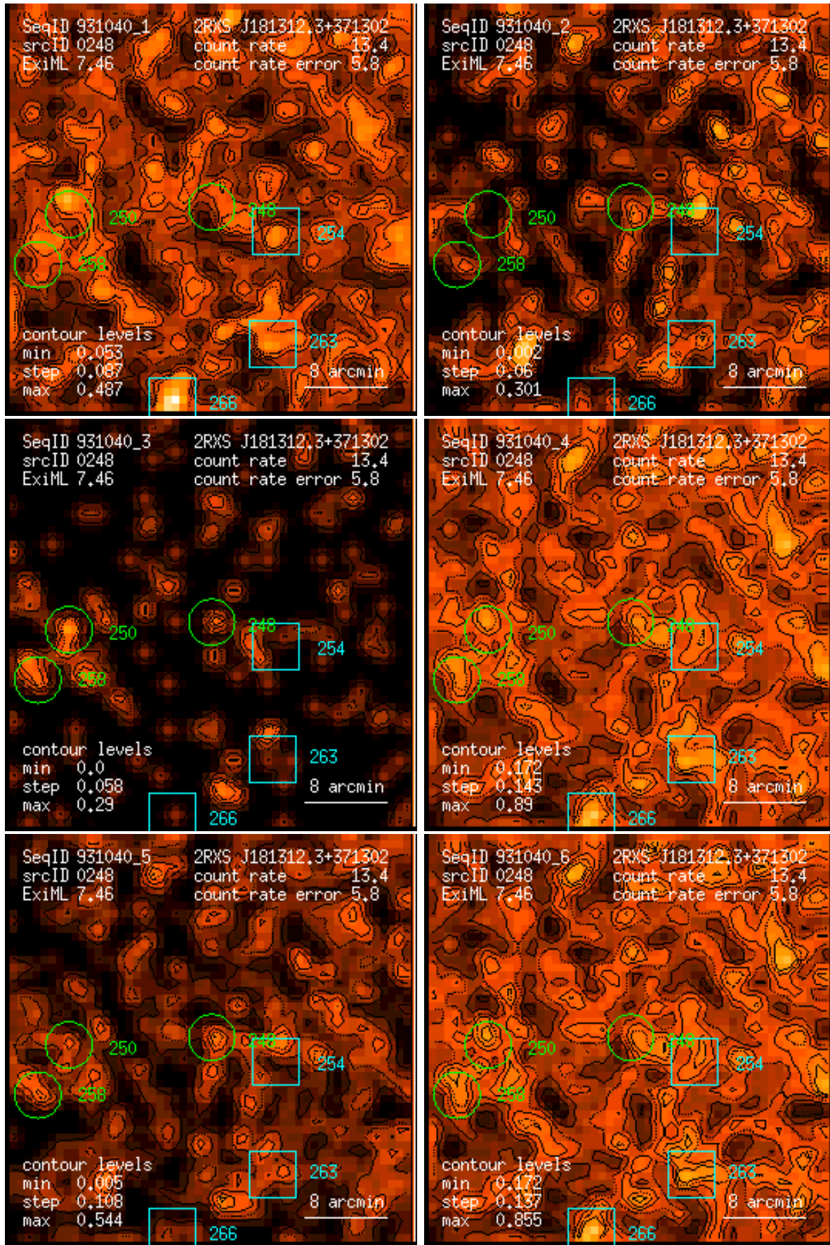
Figure 248: RASS 931040: detection 0248: band rate images, Gaussian filter: (1) PSPC channels 11 – 41, (2) 52 – 90, (3) 91 – 201, (4) 11 – 235, (5) 52 – 201, (6) 11 – 201. Broad band rates in counts/ks. Band rate contour levels in counts/ks/arcmin 2 .
