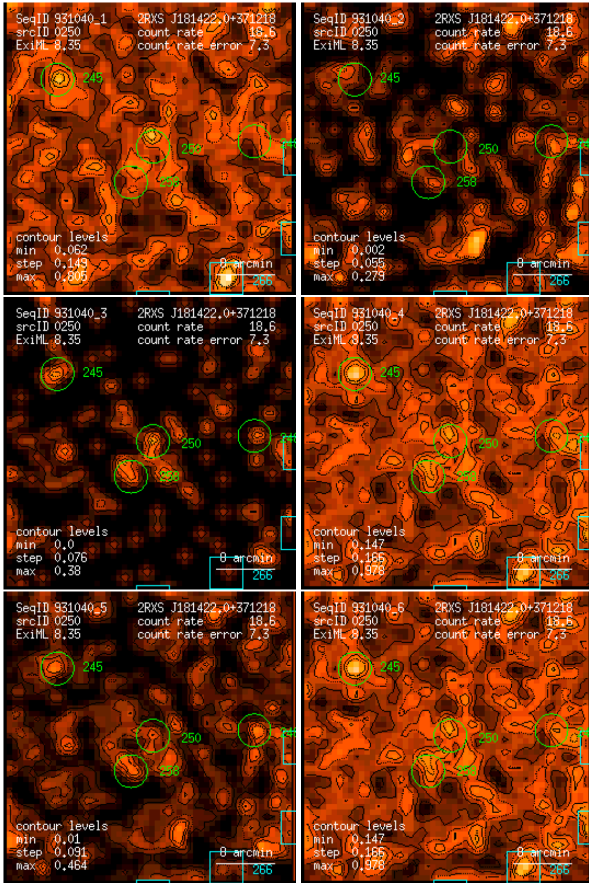
Figure 250: RASS 931040: detection 0250: band rate images, Gaussian filter: (1) PSPC channels 11 – 41, (2) 52 – 90, (3) 91 – 201, (4) 11 – 235, (5) 52 – 201, (6) 11 – 201. Broad band rates in counts/ks. Band rate contour levels in counts/ks/arcmin 2 .
