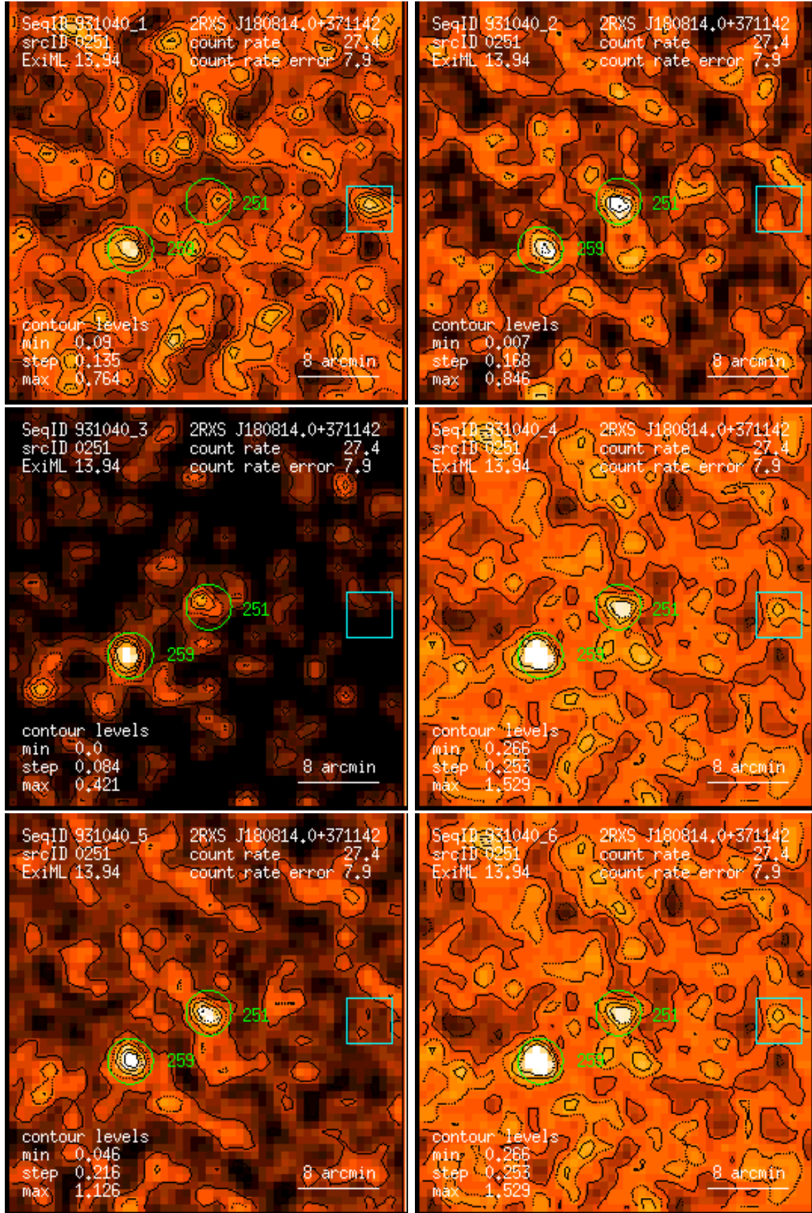
Figure 251: RASS 931040: detection 0251: band rate images, Gaussian filter: (1) PSPC channels 11 – 41, (2) 52 – 90, (3) 91 – 201, (4) 11 – 235, (5) 52 – 201, (6) 11 – 201. Broad band rates in counts/ks. Band rate contour levels in counts/ks/arcmin 2 .
