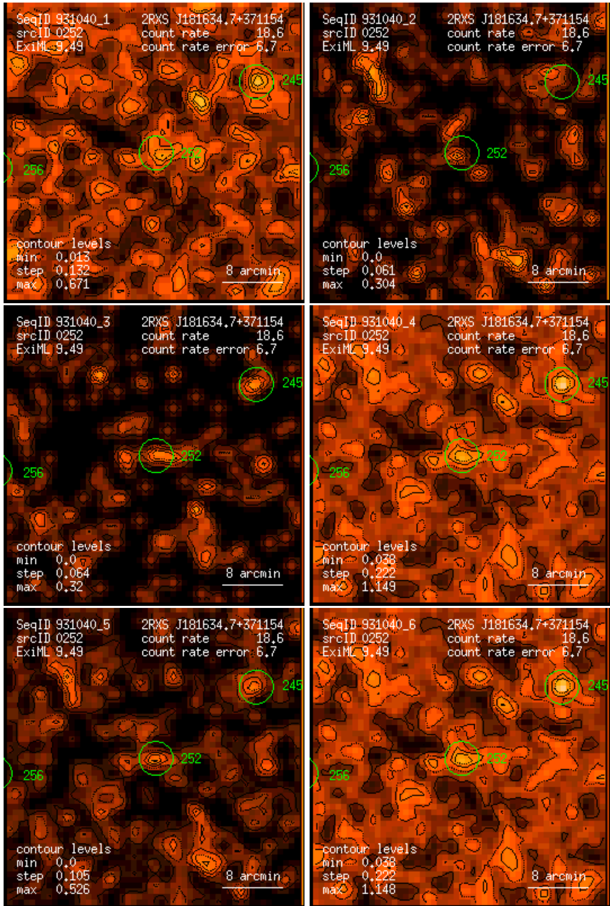
Figure 252: RASS 931040: detection 0252: band rate images, Gaussian filter: (1) PSPC channels 11 – 41, (2) 52 – 90, (3) 91 – 201, (4) 11 – 235, (5) 52 – 201, (6) 11 – 201. Broad band rates in counts/ks. Band rate contour levels in counts/ks/arcmin 2 .
