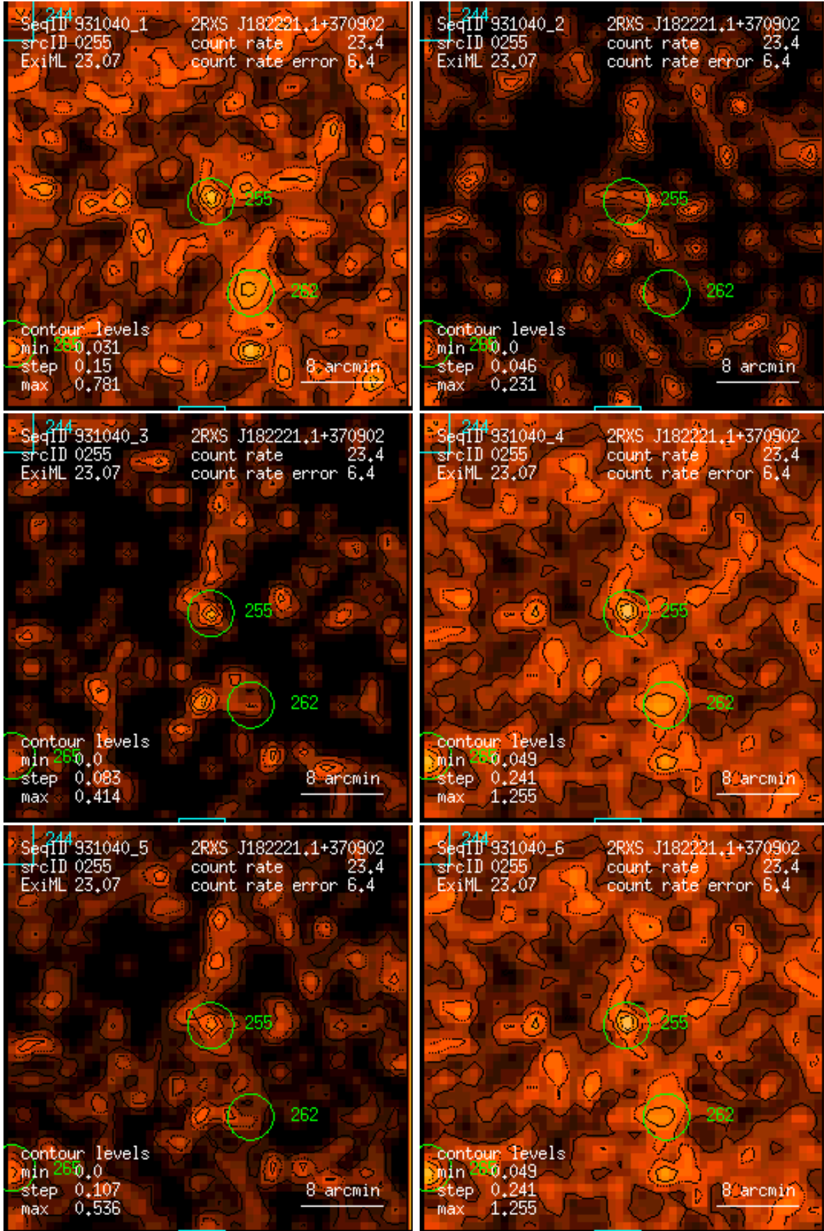
Figure 255: RASS 931040: detection 0255: band rate images, Gaussian filter: (1) PSPC channels 11 – 41, (2) 52 – 90, (3) 91 – 201, (4) 11 – 235, (5) 52 – 201, (6) 11 – 201. Broad band rates in counts/ks. Band rate contour levels in counts/ks/arcmin 2 .
