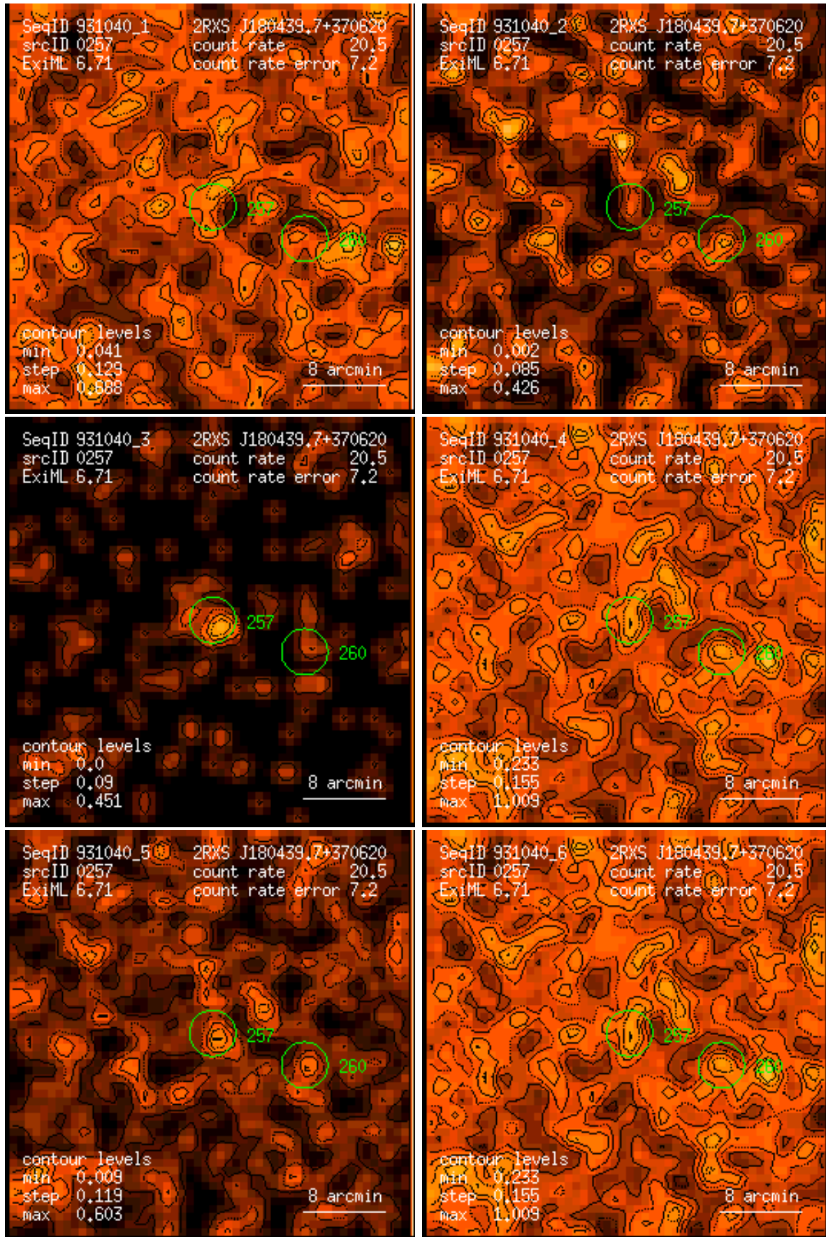
Figure 257: RASS 931040: detection 0257: band rate images, Gaussian filter: (1) PSPC channels 11 – 41, (2) 52 – 90, (3) 91 – 201, (4) 11 – 235, (5) 52 – 201, (6) 11 – 201. Broad band rates in counts/ks. Band rate contour levels in counts/ks/arcmin 2 .
