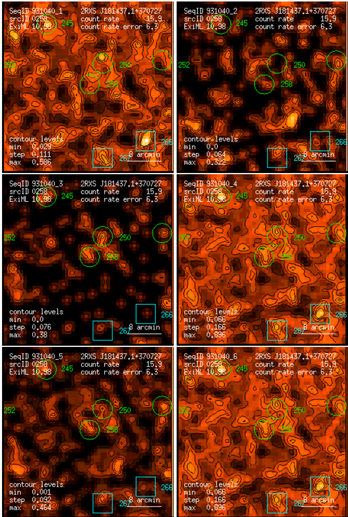
Figure 258: RASS 931040: detection 0258: band rate images, Gaussian filter: (1) PSPC channels 11 – 41, (2) 52 – 90, (3) 91 – 201, (4) 11 – 235, (5) 52 – 201, (6) 11 – 201. Broad band rates in counts/ks. Band rate contour levels in counts/ks/arcmin 2 .
