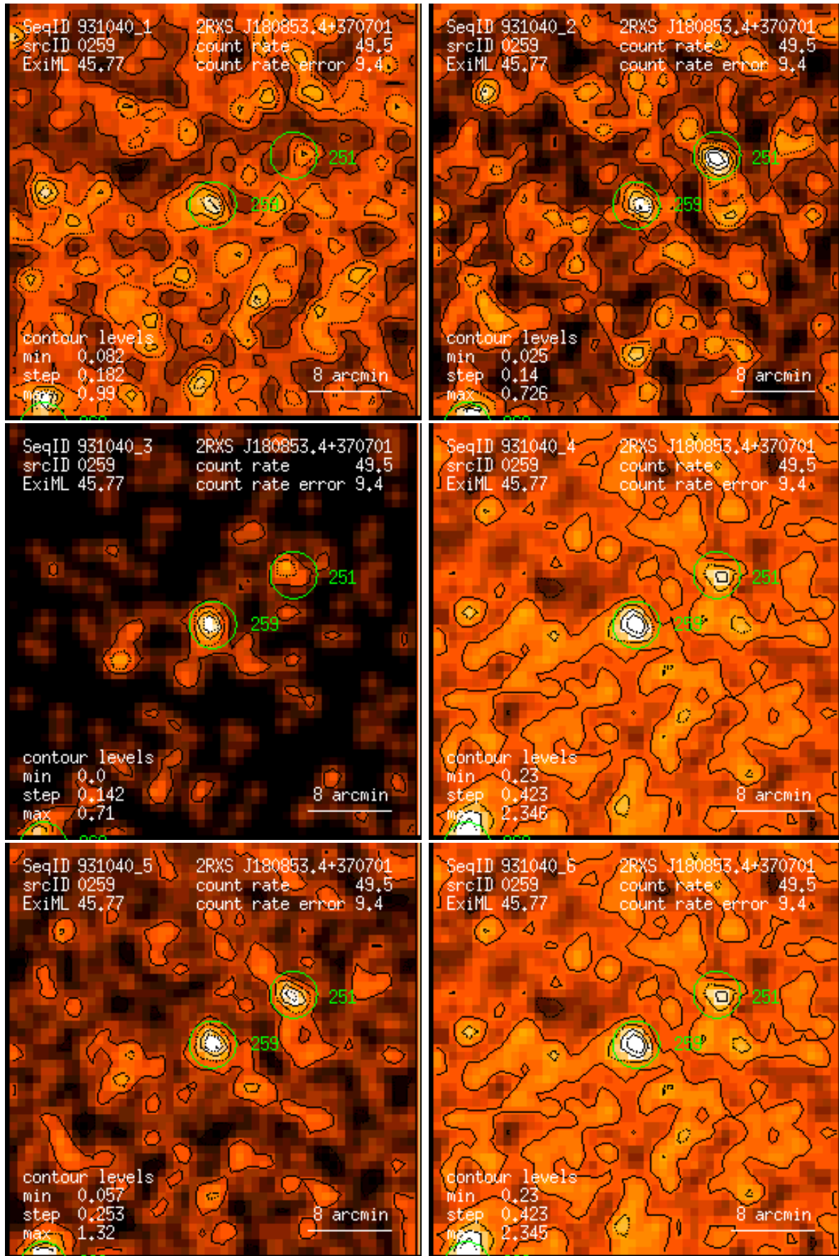
Figure 259: RASS 931040: detection 0259: band rate images, Gaussian filter: (1) PSPC channels 11 – 41, (2) 52 – 90, (3) 91 – 201, (4) 11 – 235, (5) 52 – 201, (6) 11 – 201. Broad band rates in counts/ks. Band rate contour levels in counts/ks/arcmin 2 .
