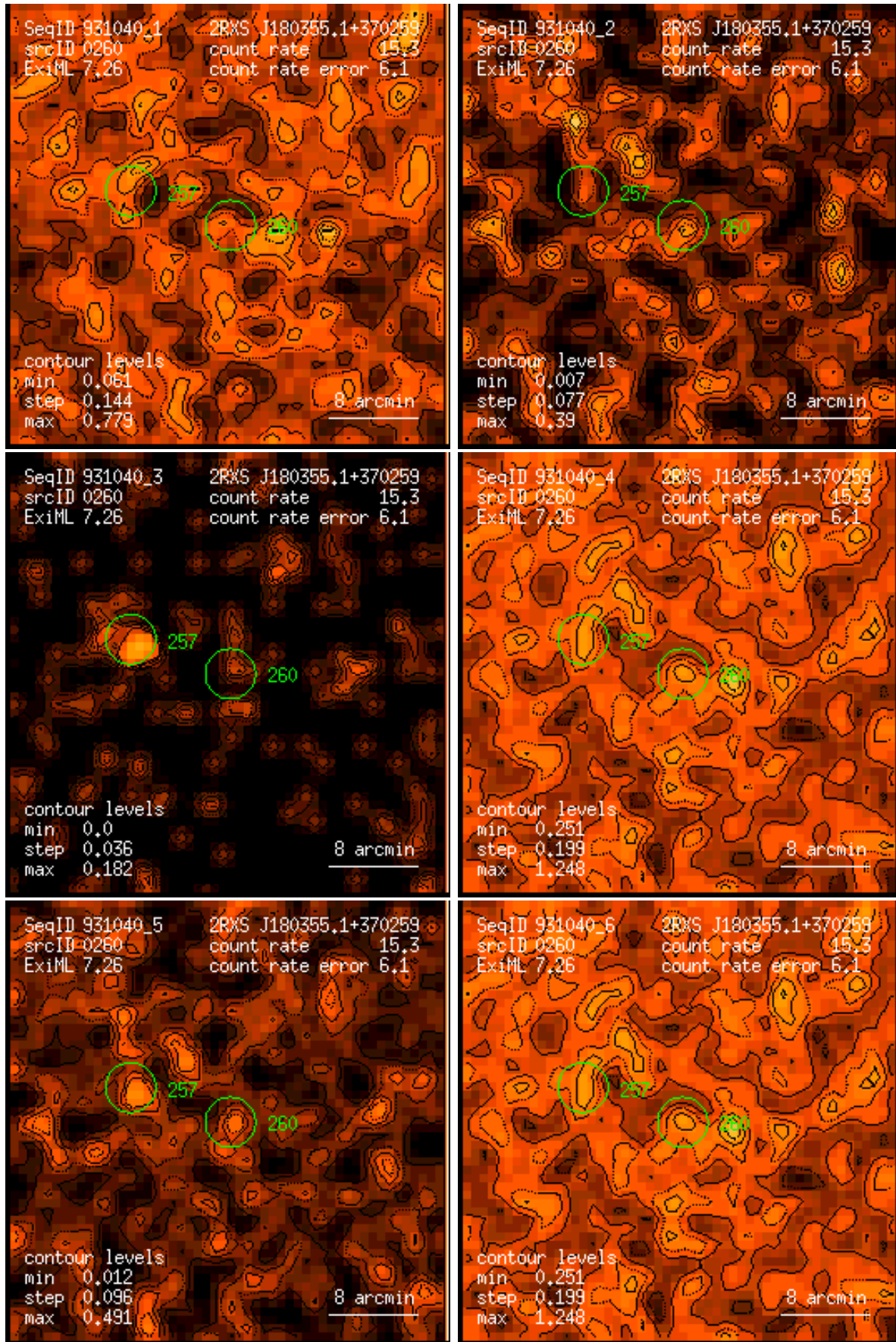
Figure 260: RASS 931040: detection 0260: band rate images, Gaussian filter: (1) PSPC channels 11 – 41, (2) 52 – 90, (3) 91 – 201, (4) 11 – 235, (5) 52 – 201, (6) 11 – 201. Broad band rates in counts/ks. Band rate contour levels in counts/ks/arcmin 2 .
