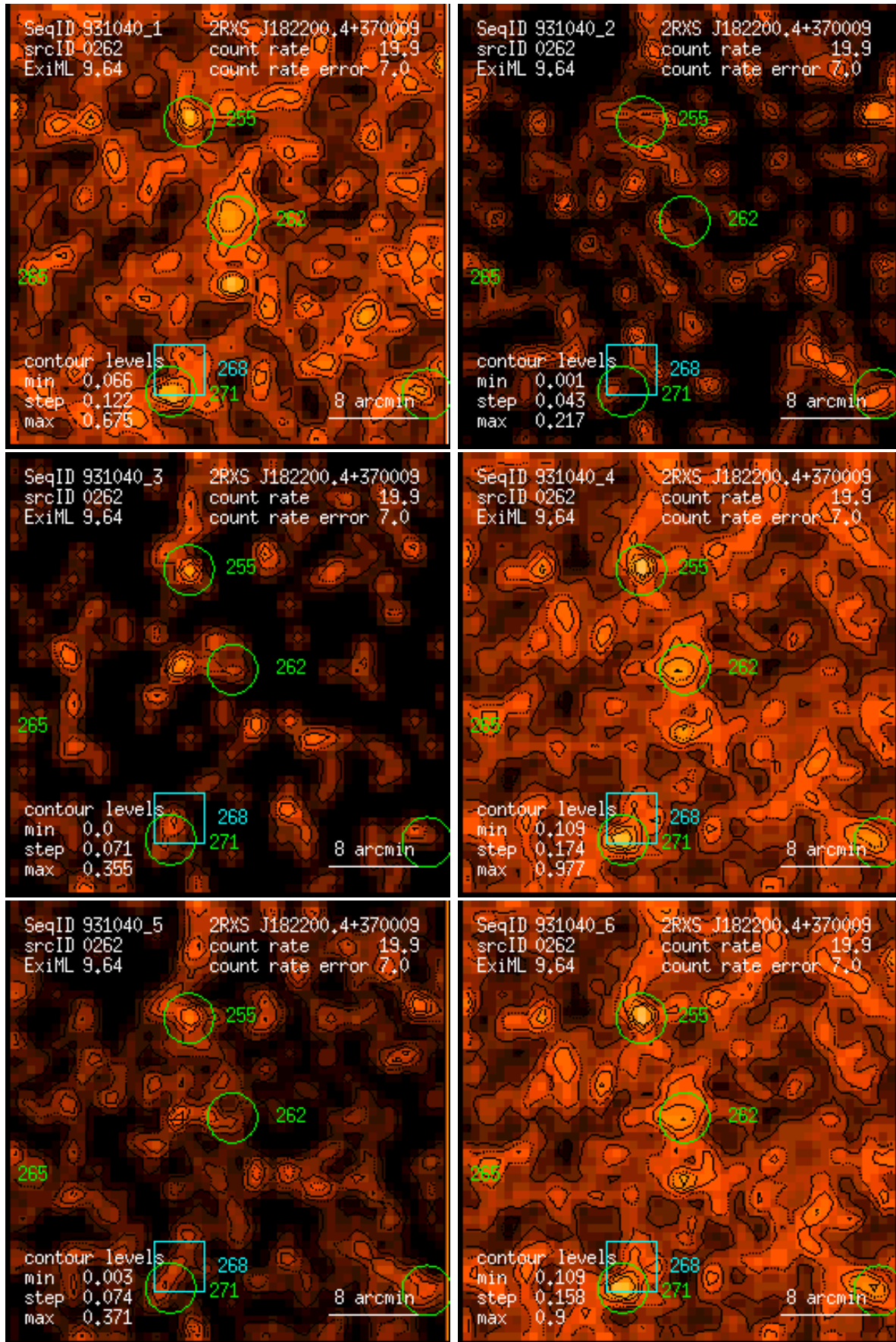
Figure 262: RASS 931040: detection 0262: band rate images, Gaussian filter: (1) PSPC channels 11 – 41, (2) 52 – 90, (3) 91 – 201, (4) 11 – 235, (5) 52 – 201, (6) 11 – 201. Broad band rates in counts/ks. Band rate contour levels in counts/ks/arcmin 2 .
