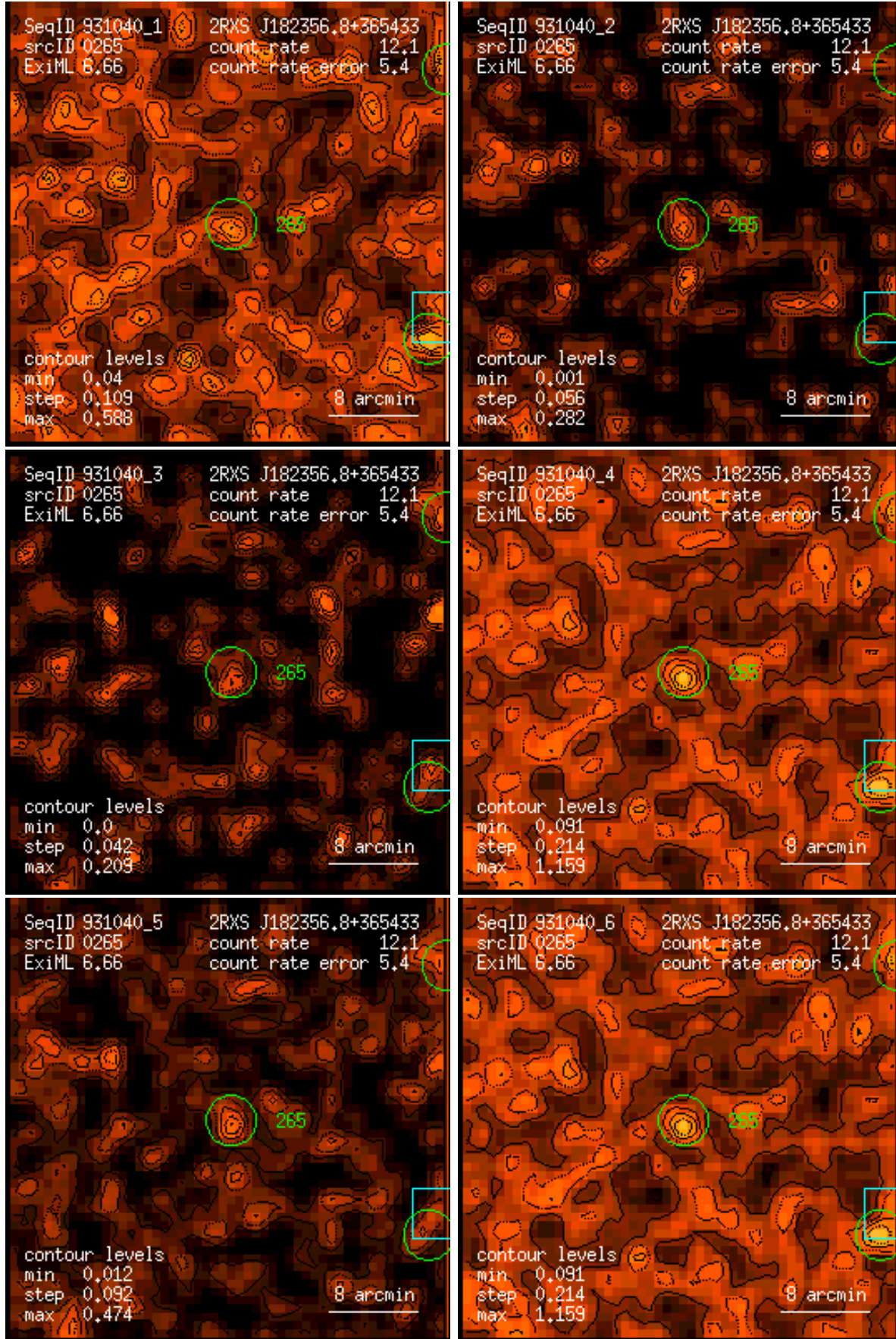
Figure 265: RASS 931040: detection 0265: band rate images, Gaussian filter: (1) PSPC channels 11 – 41, (2) 52 – 90, (3) 91 – 201, (4) 11 – 235, (5) 52 – 201, (6) 11 – 201. Broad band rates in counts/ks. Band rate contour levels in counts/ks/arcmin 2 .
