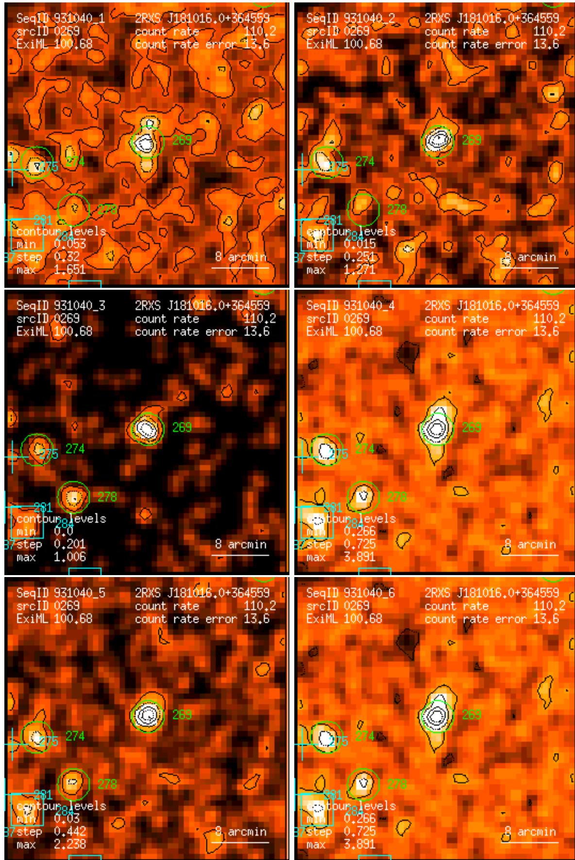
Figure 269: RASS 931040: detection 0269: band rate images, Gaussian filter: (1) PSPC channels 11 – 41, (2) 52 – 90, (3) 91 – 201, (4) 11 – 235, (5) 52 – 201, (6) 11 – 201. Broad band rates in counts/ks. Band rate contour levels in counts/ks/arcmin 2 .
