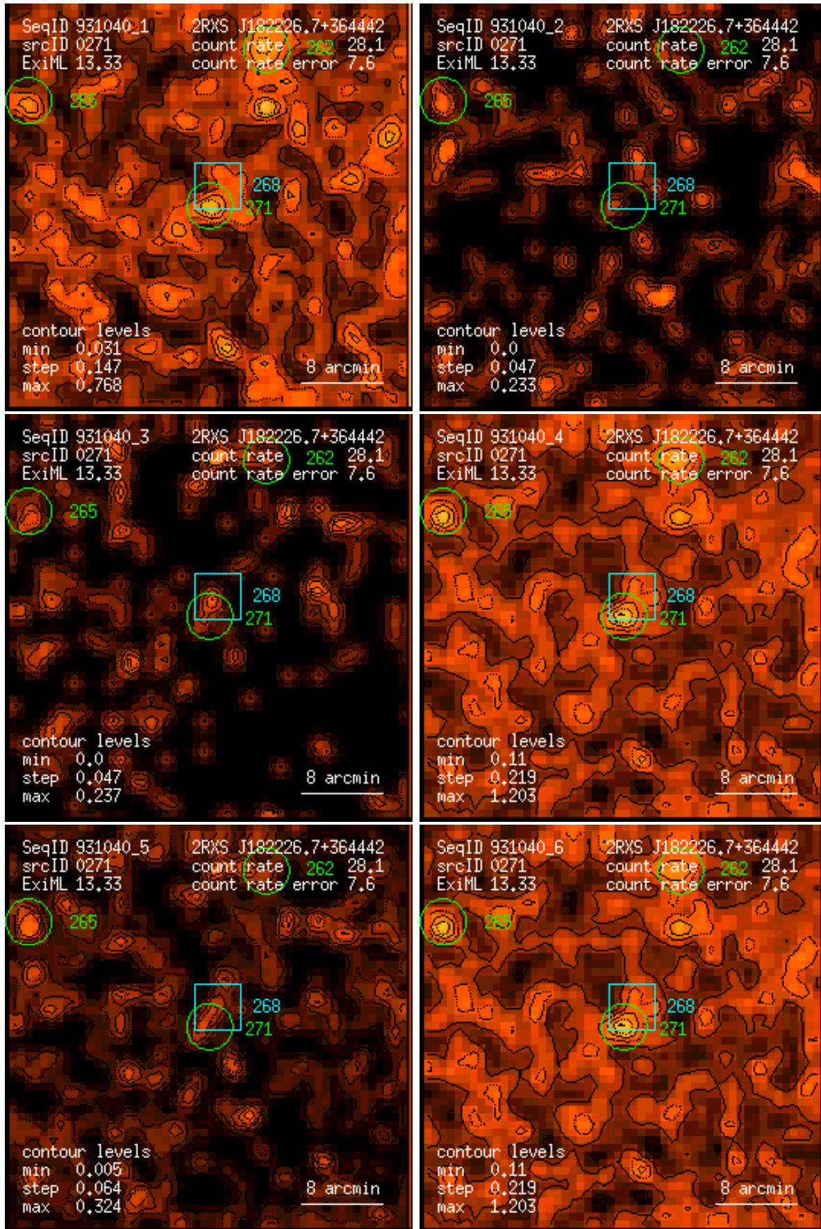
Figure 271: RASS 931040: detection 0271: band rate images, Gaussian filter: (1) PSPC channels 11 – 41, (2) 52 – 90, (3) 91 – 201, (4) 11 – 235, (5) 52 – 201, (6) 11 – 201. Broad band rates in counts/ks. Band rate contour levels in counts/ks/arcmin 2 .
