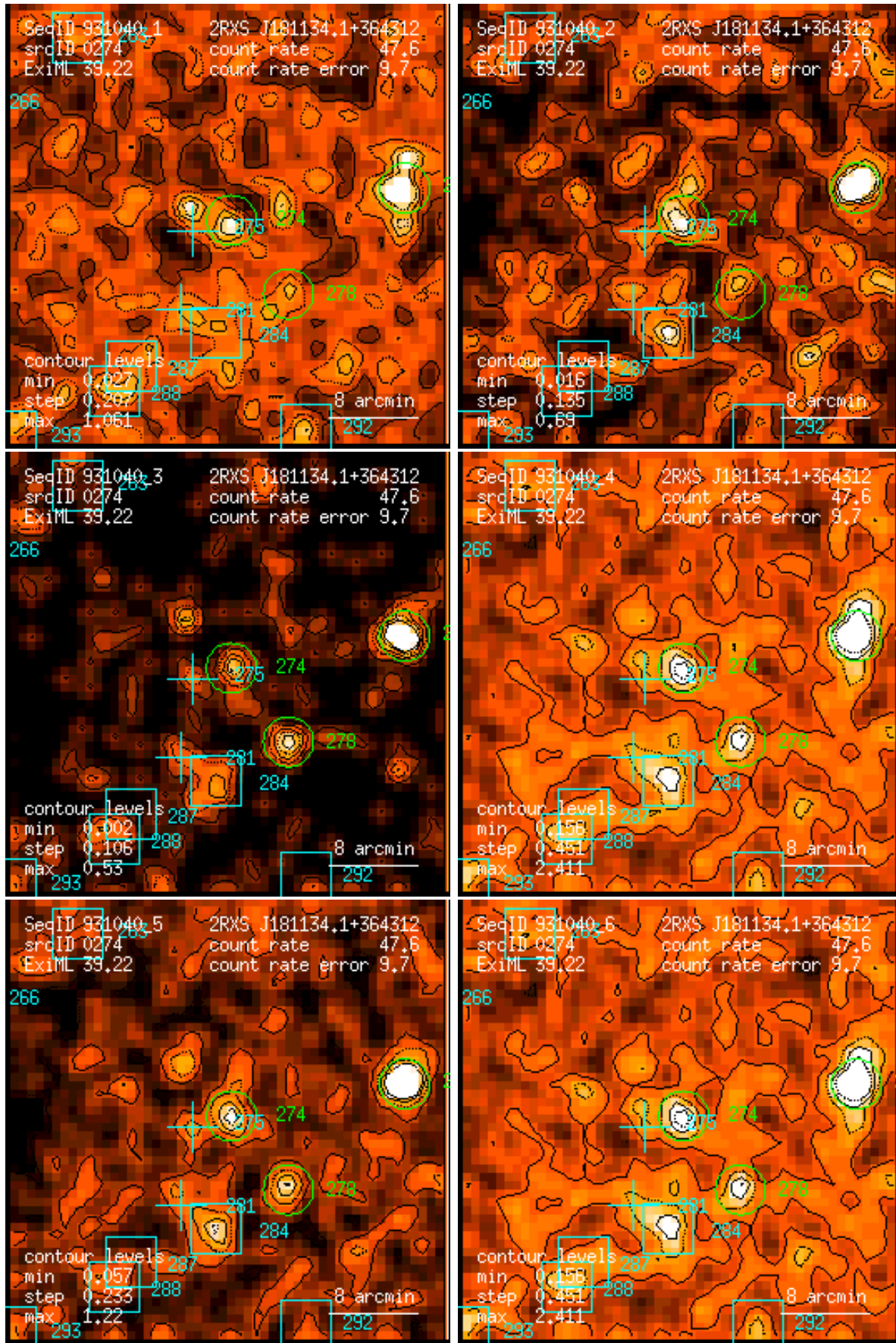
Figure 274: RASS 931040: detection 0274: band rate images, Gaussian filter: (1) PSPC channels 11 – 41, (2) 52 – 90, (3) 91 – 201, (4) 11 – 235, (5) 52 – 201, (6) 11 – 201. Broad band rates in counts/ks. Band rate contour levels in counts/ks/arcmin 2 .
