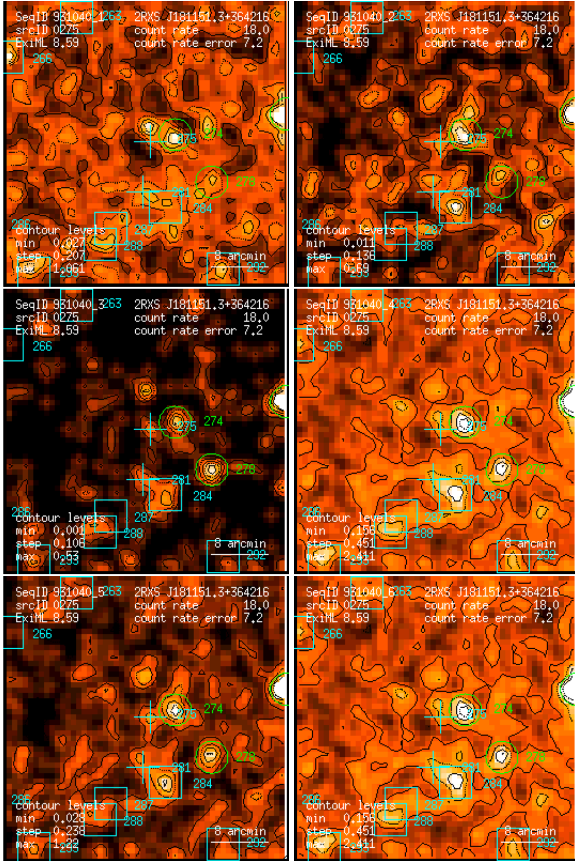
Figure 275: RASS 931040: detection 0275: band rate images, Gaussian filter: (1) PSPC channels 11 – 41, (2) 52 – 90, (3) 91 – 201, (4) 11 – 235, (5) 52 – 201, (6) 11 – 201. Broad band rates in counts/ks. Band rate contour levels in counts/ks/arcmin 2 .
