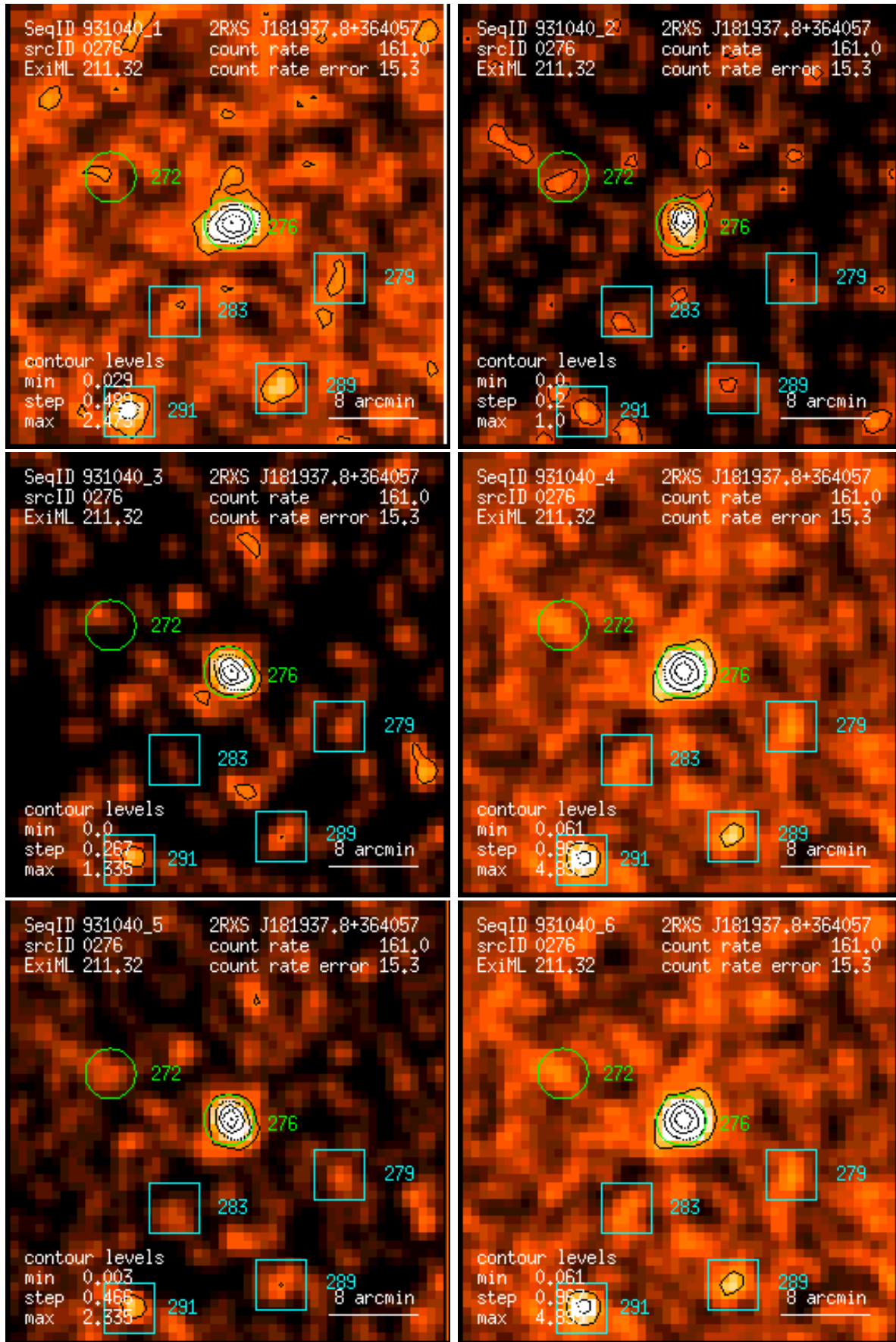
Figure 276: RASS 931040: detection 0276: band rate images, Gaussian filter: (1) PSPC channels 11 – 41, (2) 52 – 90, (3) 91 – 201, (4) 11 – 235, (5) 52 – 201, (6) 11 – 201. Broad band rates in counts/ks. Band rate contour levels in counts/ks/arcmin 2 .
