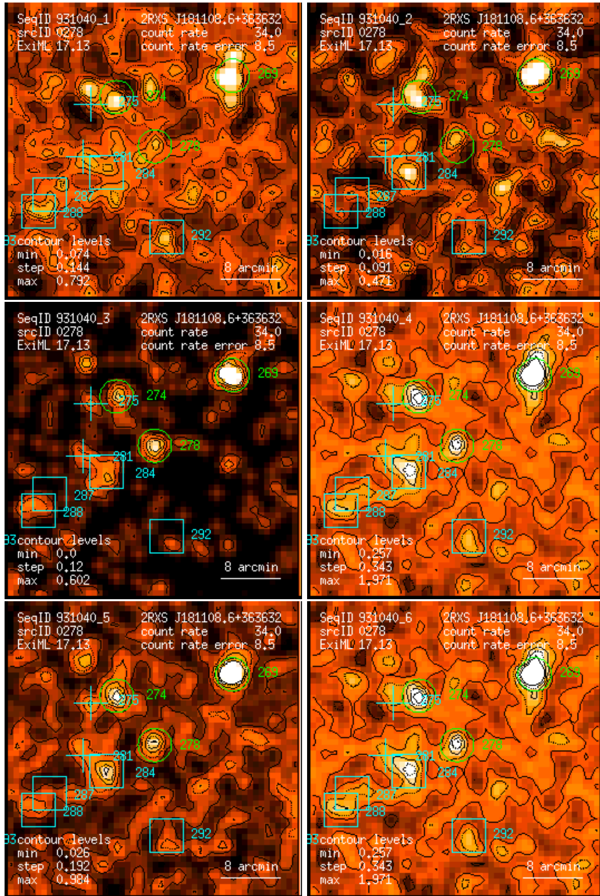
Figure 278: RASS 931040: detection 0278: band rate images, Gaussian filter: (1) PSPC channels 11 – 41, (2) 52 – 90, (3) 91 – 201, (4) 11 – 235, (5) 52 – 201, (6) 11 – 201. Broad band rates in counts/ks. Band rate contour levels in counts/ks/arcmin 2 .
