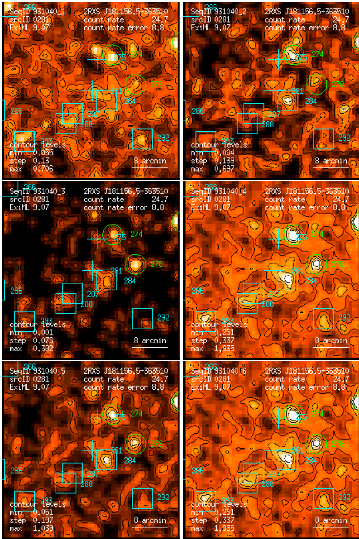
Figure 281: RASS 931040: detection 0281: band rate images, Gaussian filter: (1) PSPC channels 11 – 41, (2) 52 – 90, (3) 91 – 201, (4) 11 – 235, (5) 52 – 201, (6) 11 – 201. Broad band rates in counts/ks. Band rate contour levels in counts/ks/arcmin 2 .
